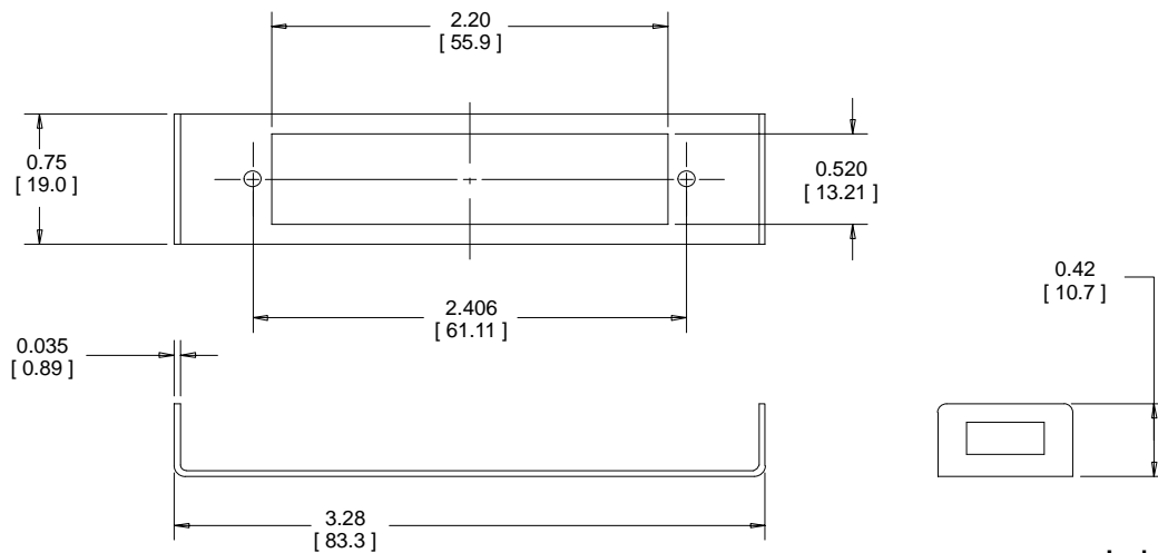
Latch Bracket
