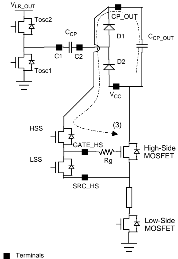
Figure 9. High-Side Gate Driver
