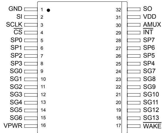
Figure 3. 33975 Terminal Connections
