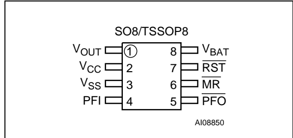
Figure 6. STM704/806 Connections
