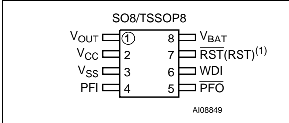
Figure 5. STM690/802/804/805 Connections
