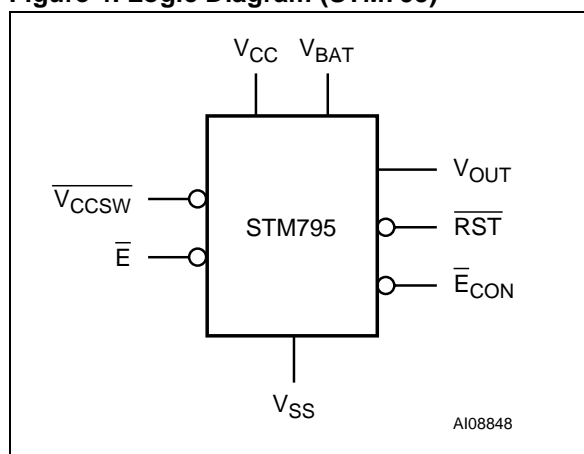
Figure 4. Logic Diagram (STM795)
