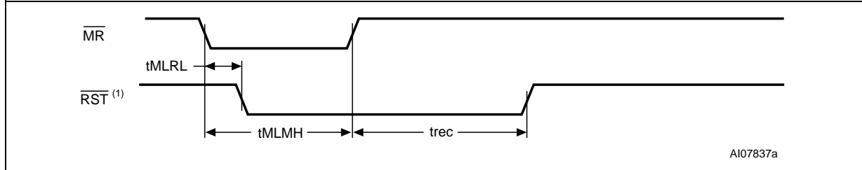
Figure 37. \overline{\text{MR}} Timing Waveform
