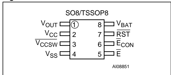
Figure 7. STM795 Connections
