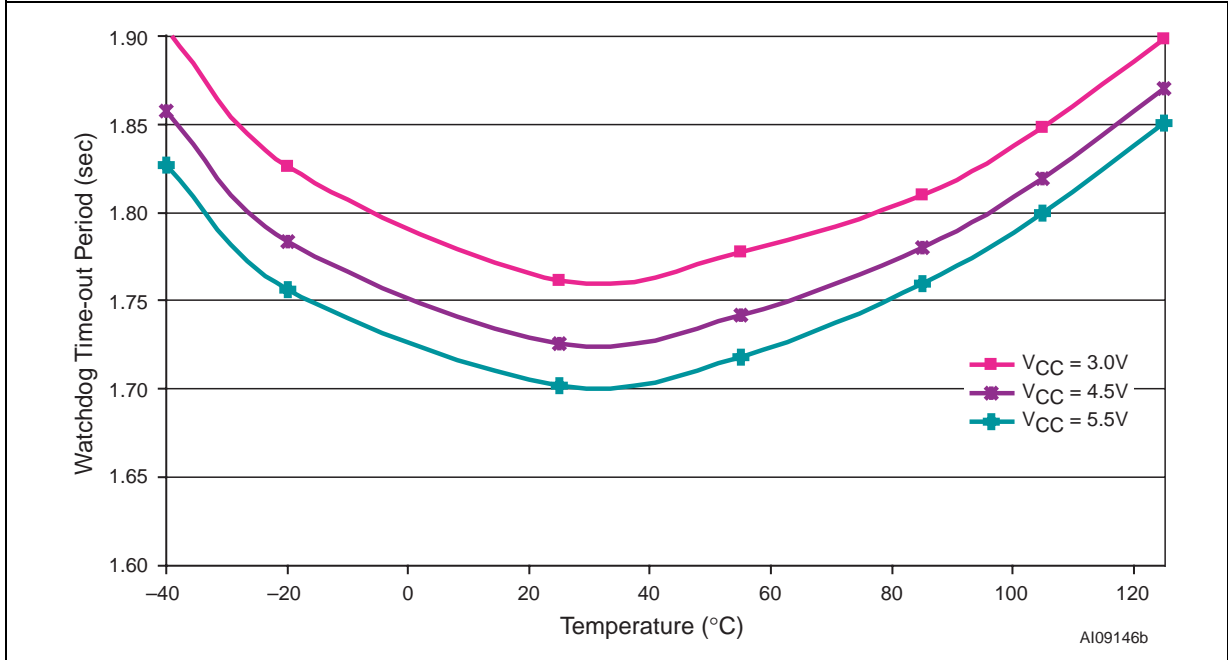
Figure 24. Watchdog Time-out Period vs. Temperature
