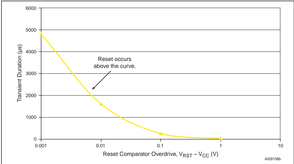
Figure 33. Maximum Transient Duration vs. Reset Threshold Overdrive
