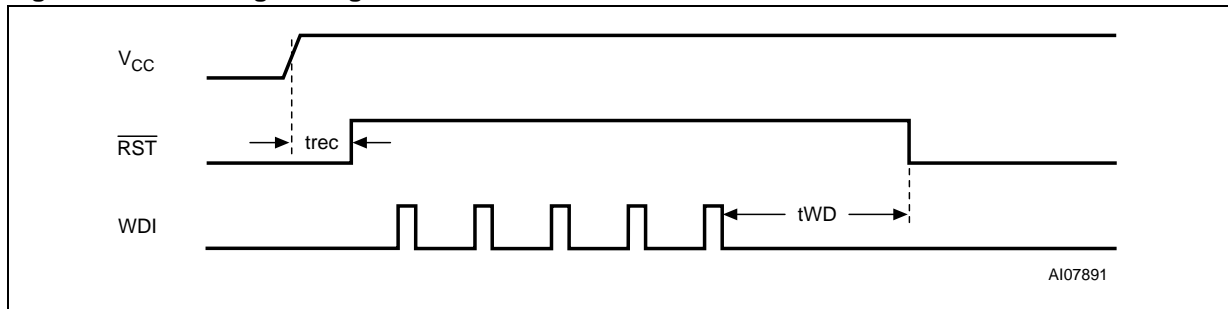
Figure 38. Watchdog Timing
