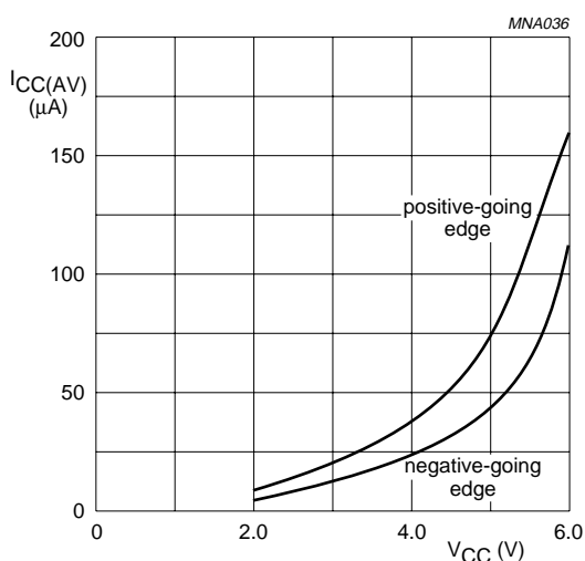
Fig.14 Average I_{CC} for AHC1G Schmitt-trigger devices; linear change of V_I between 0.1V_{CC} to 0.9V_{CC} .
