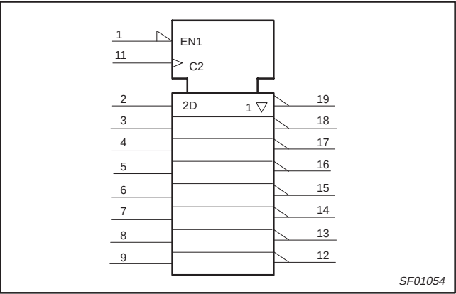
IEC/IEEE SYMBOL – 74ALS564A
