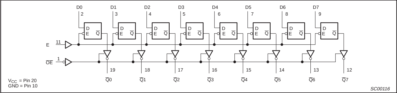
LOGIC DIAGRAM – 74ALS563A
