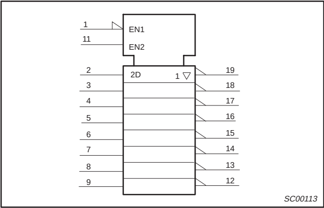
IEC/IEEE SYMBOL – 74ALS563A
