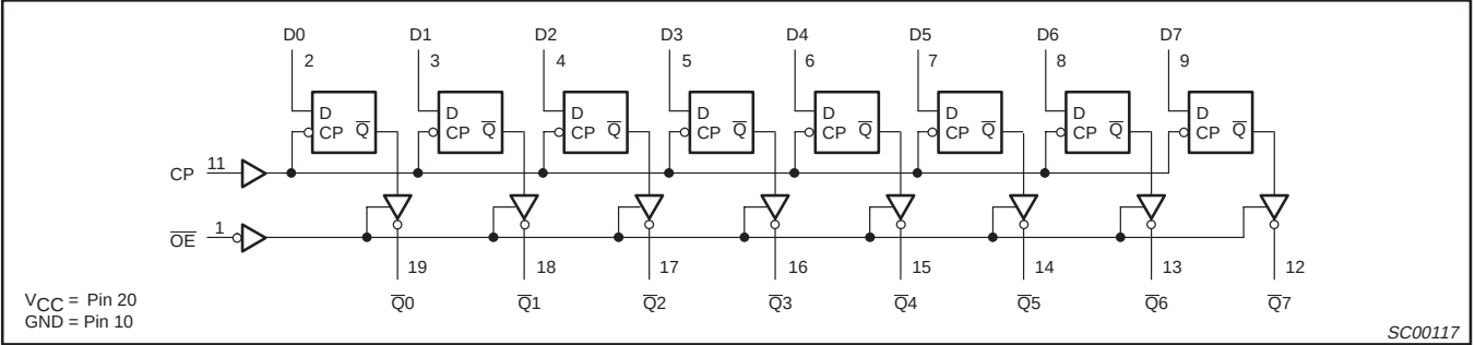
LOGIC DIAGRAM – 74ALS564A
