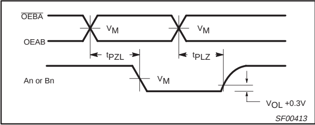
Waveform 4. 3-State Output Enable Time to Low Level and Disable Time from Low Level
