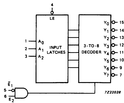
Fig.2 Logic symbol.
