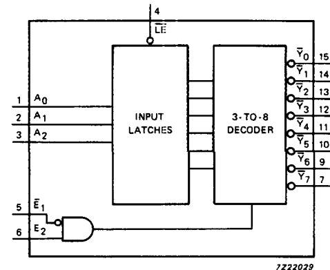
Fig.4 Functional diagram.
