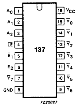
Fig.1 Pin configuration.
