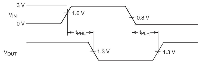
Figure 2. AC Waveforms
