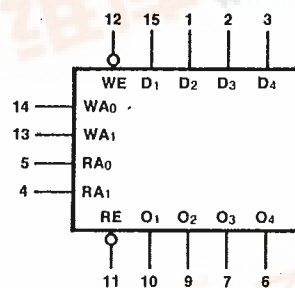
LOGIC SYMBOL
