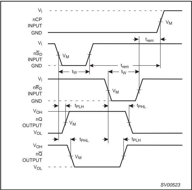
Figure 2. Set (nS) and reset (nR) input to output (nQ, nQ) propagation delays, the set and reset pulse widths and the nR, nS to nCP removal time.
