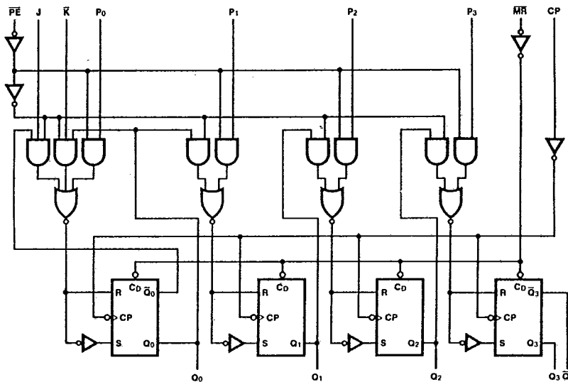
LOGIC DIAGRAM
