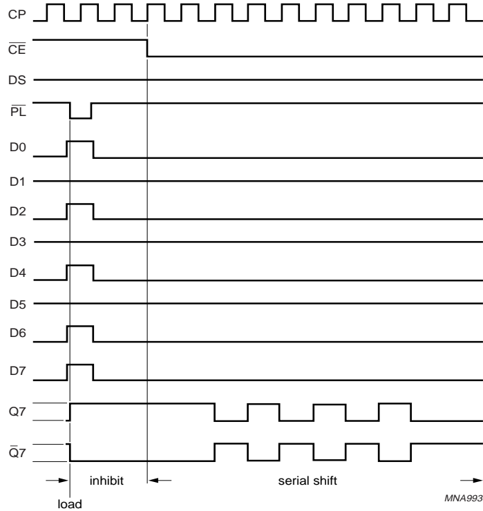
Fig.6 Timing diagram.
