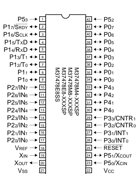
Outline 42P4B (Note 1) 42S1B-A (Window)
