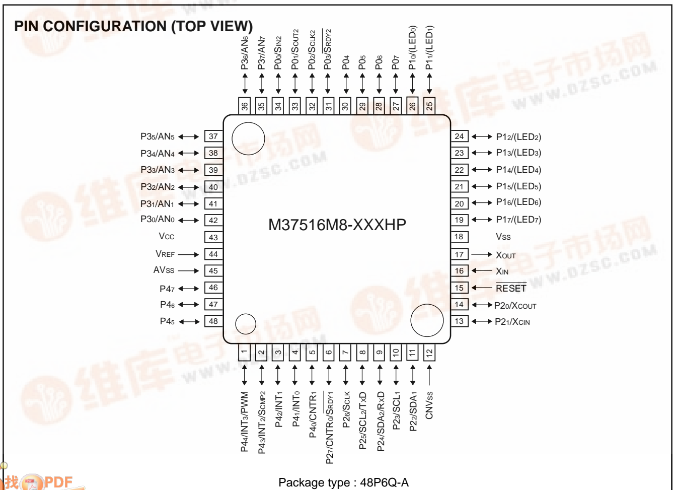
Fig. 3 M37516F8HP pin configuration
