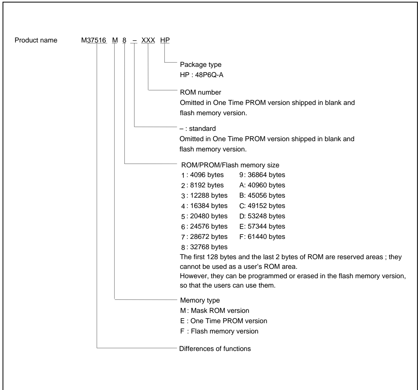
Fig. 3 Part numbering
