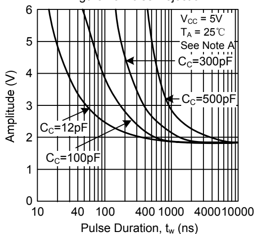
Figure 13 Noise Rejection
