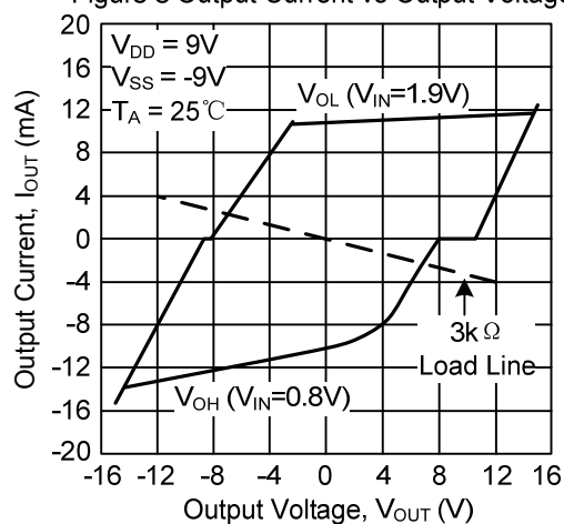
Figure 8 Output Current vs Output Voltage
