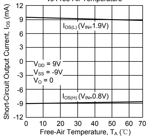
Figure 9 Short-Circuit Output Current vs Free-Air Temperature
