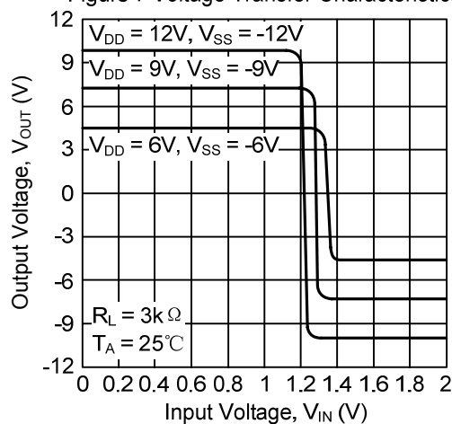
Figure 7 Voltage Transfer Characteristics
