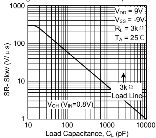
Figure 10 Slow Rate vs Load Capacitance
