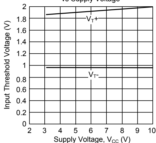
Figure 12 Input Threshold Voltage vs Supply Voltage
