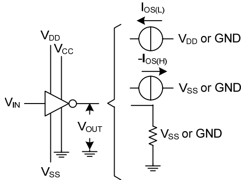
Figure. 1 For V_{OH} , V_{OL} , I_{OS(H)} , I_{OS(L)}
