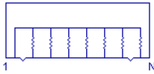
Bussed SRT Schematic 1
