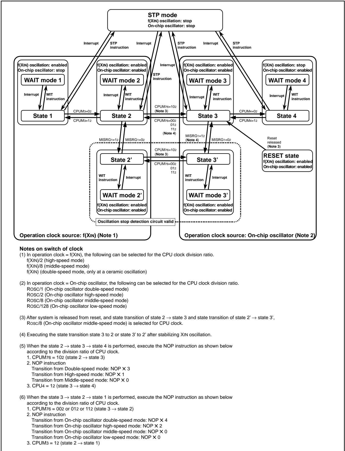
Fig. 78 State transition
