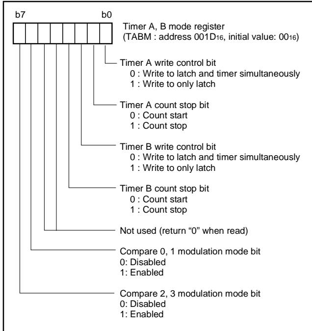
Fig. 26 Structure of timer A, B mode register
