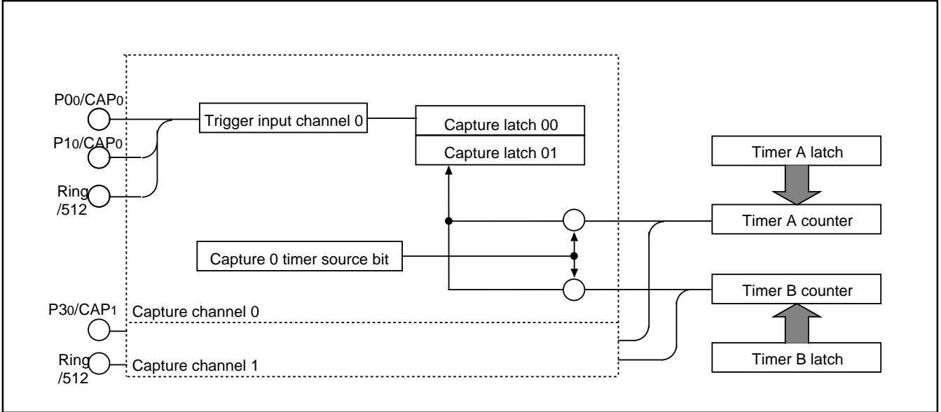
Fig. 45 Block diagram of input capture
