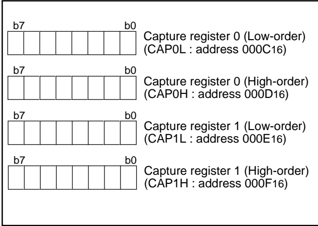
Fig. 43 Structure of capture software trigger register
