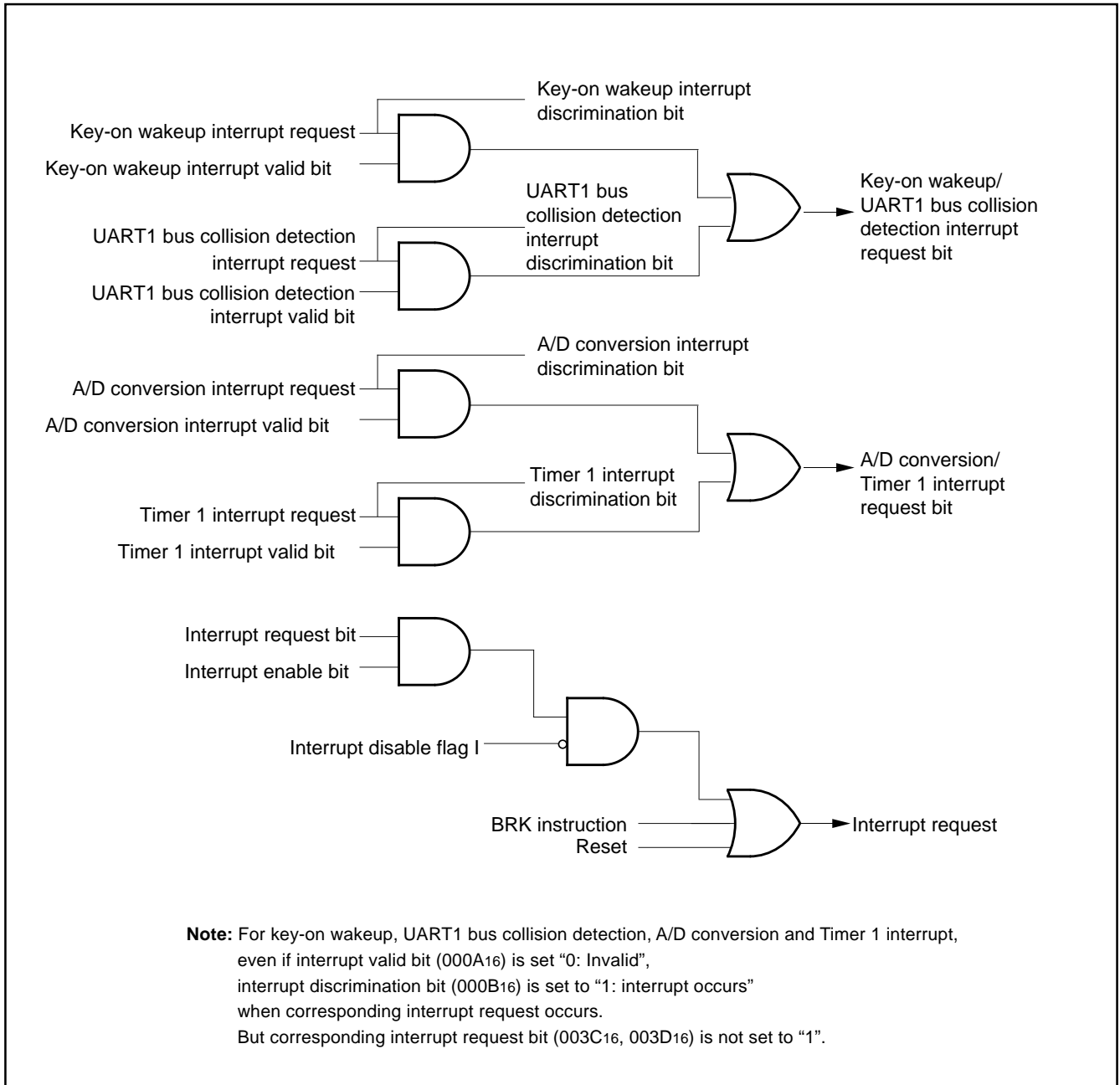
Fig. 20 Interrupt control
