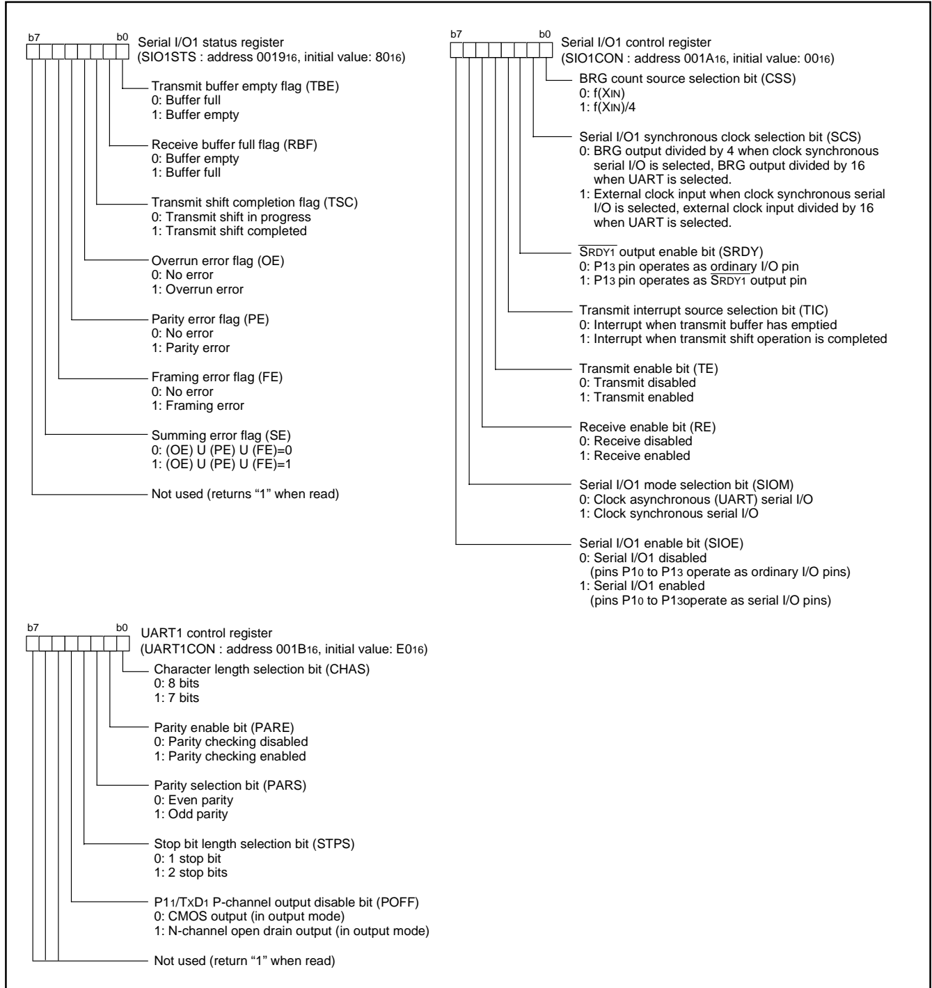
Fig. 53 Structure of serial I/O1-related registers
