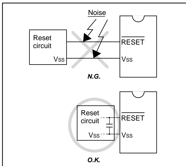
Fig. 85 Wiring for the \overline{\text{RESET}} pin
