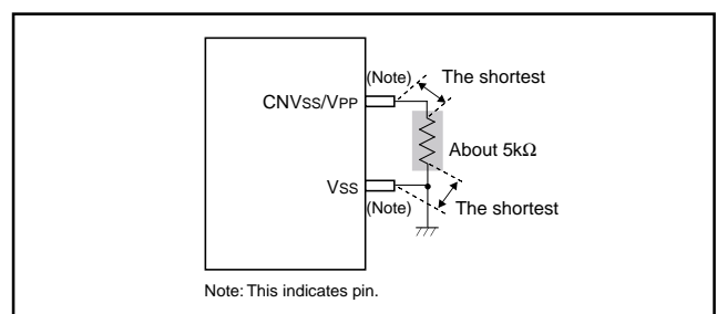
Fig. 87 Wiring for the Vpp pin of the QzPROM
