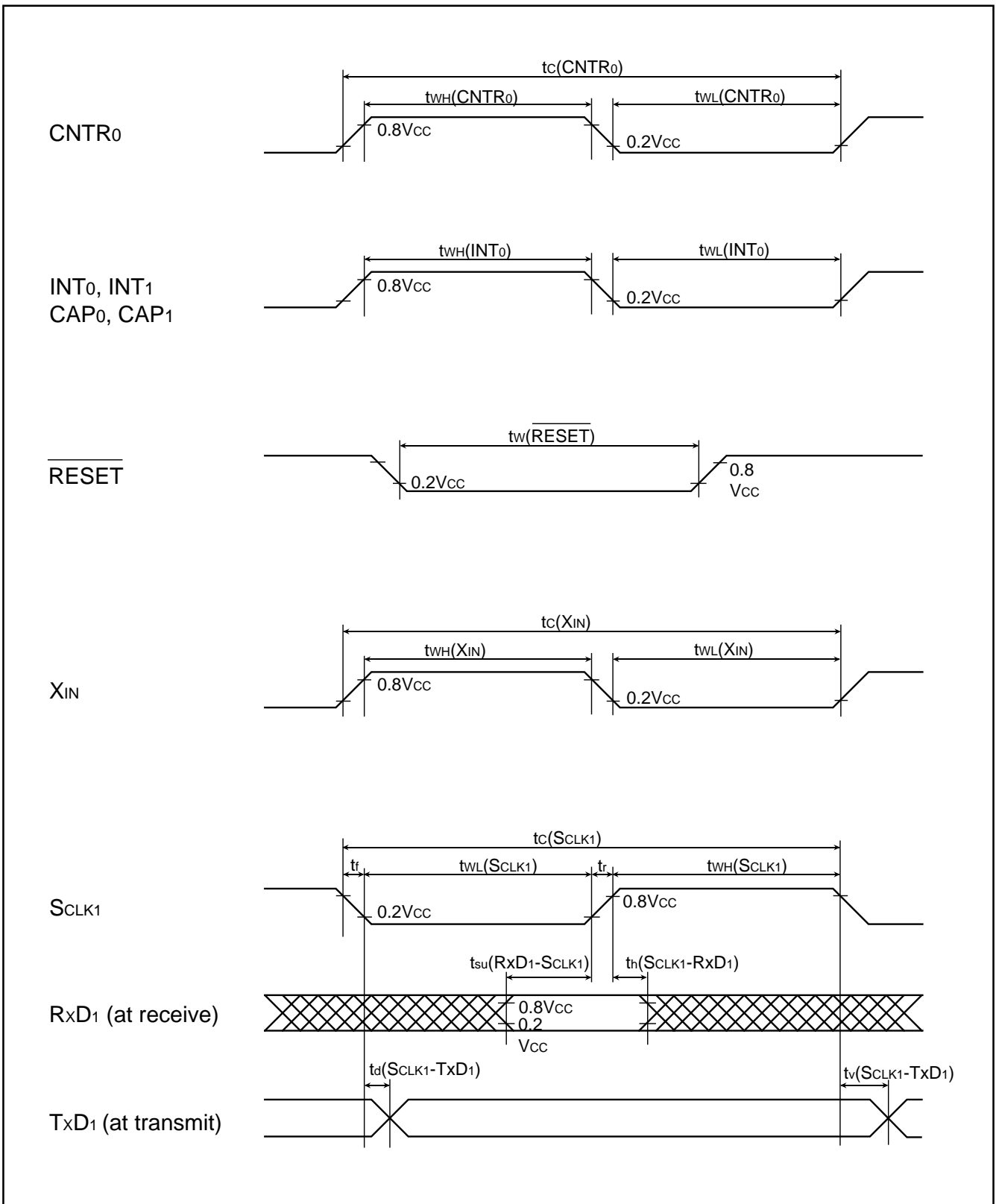
Fig. 95 Timing chart
