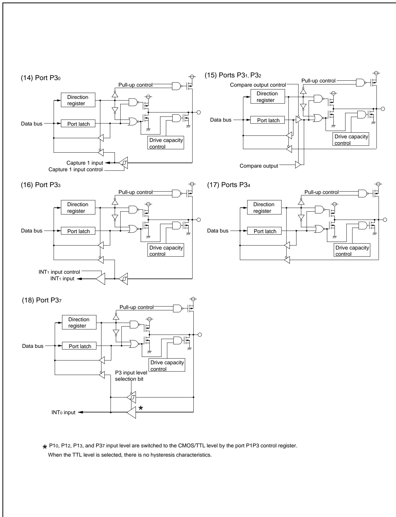
Fig. 19 Block diagram of ports (3)
