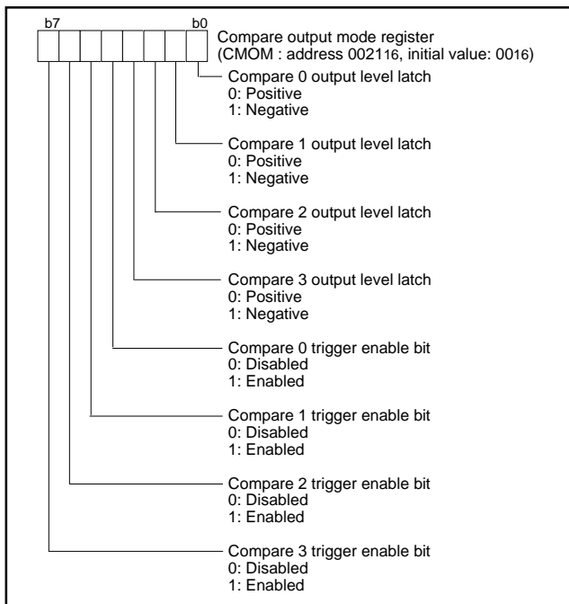
Fig. 33 Structure of compare output mode register
