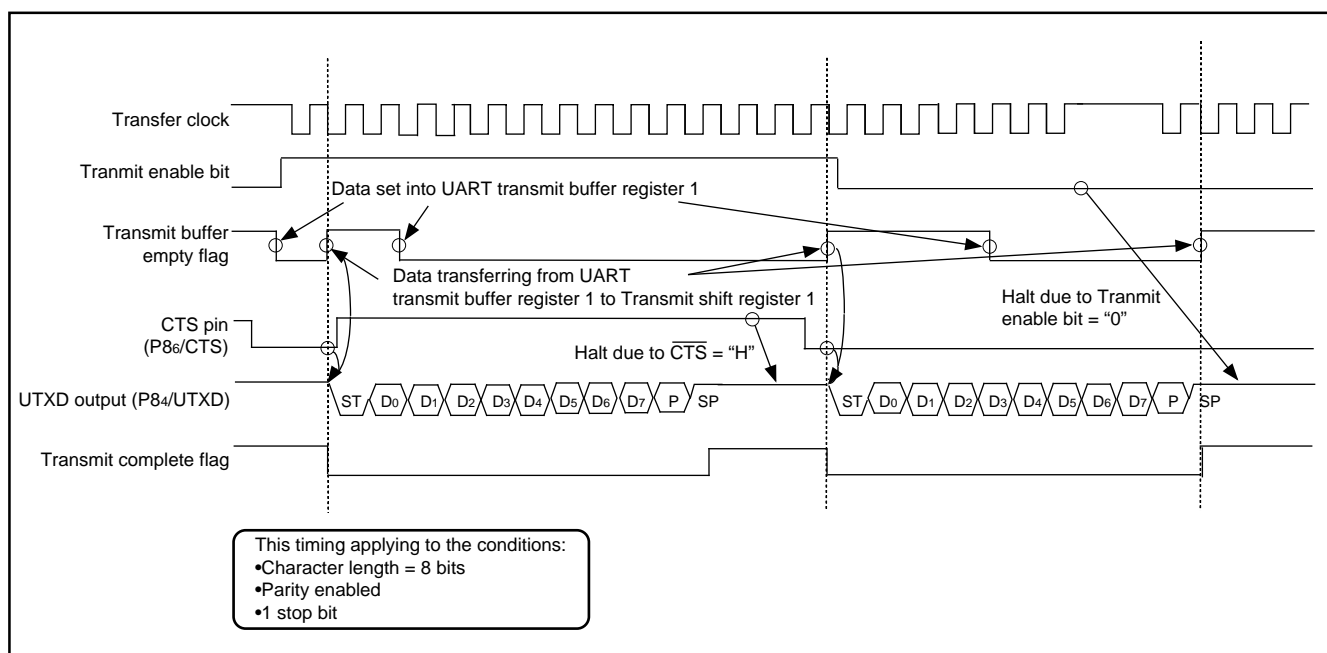
Fig. 25 UART transmit timing ( \overline{\text{CTS}} function enabled)
