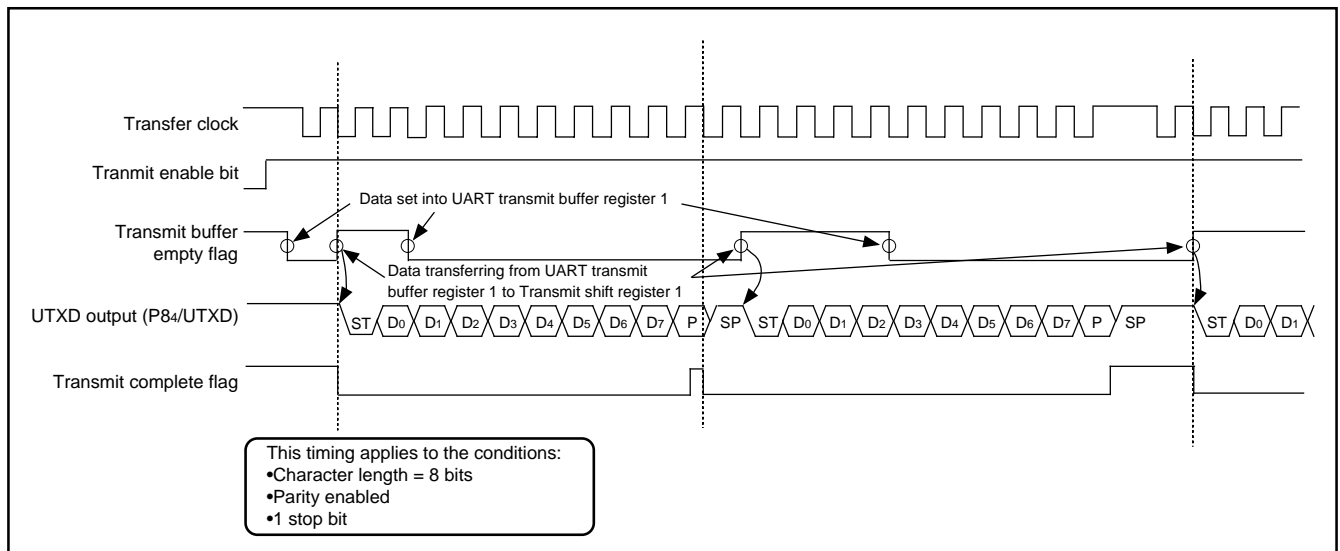
Fig. 26 UART transmit timing ( \overline{\text{CTS}} function disabled)
