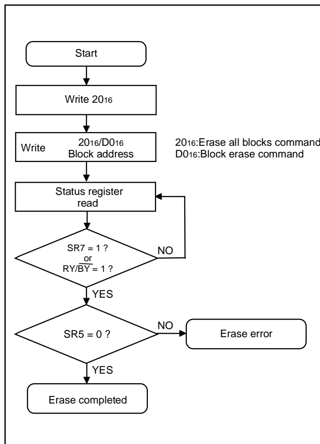
Fig. 82 Erase flowchart
