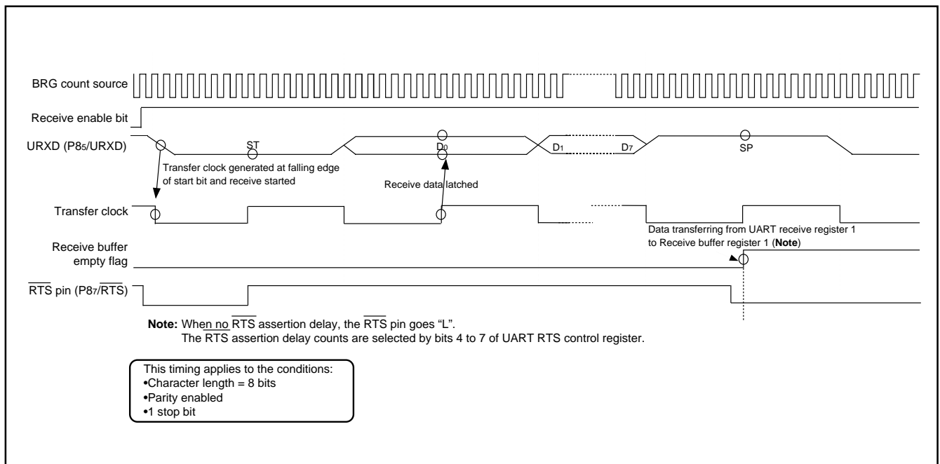
Fig. 27 UART receiving timing ( \overline{\text{RTS}} function enabled)
