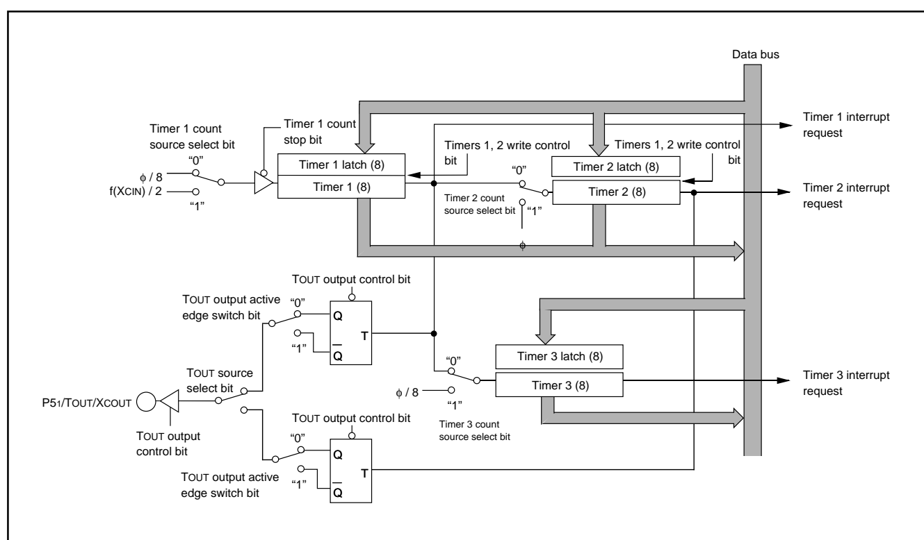
Fig. 19 Timer block diagram
