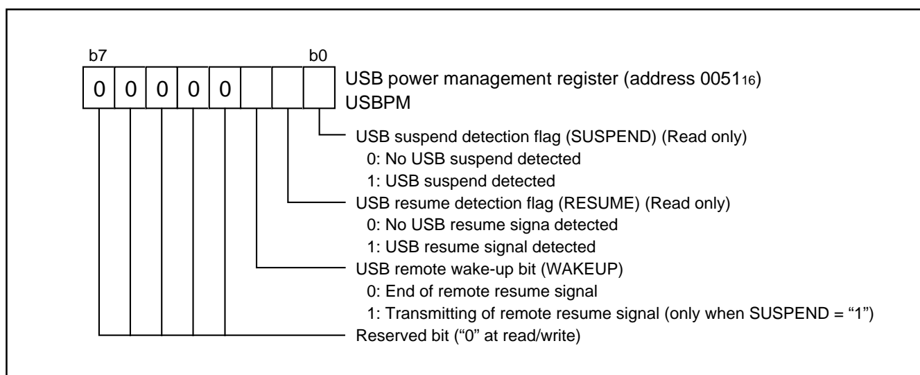
Fig. 37 Structure of USB power management register
