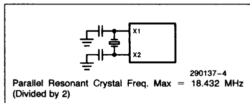
Figure 4. Crystal Oscillator
