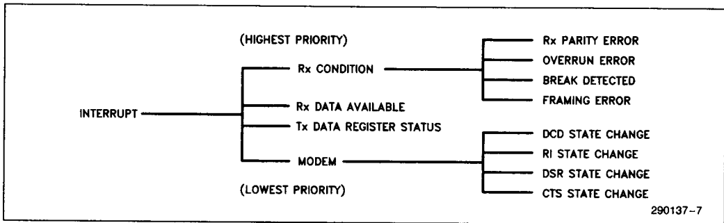
Figure 8. Interrupt Structure
