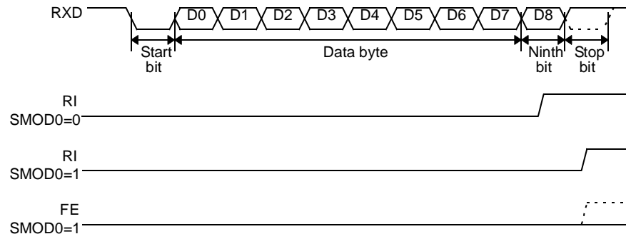
Figure 19. UART Timings in Modes 2 and 3
