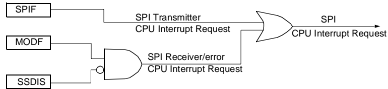
Figure 31. SPI Interrupt Requests Generation
