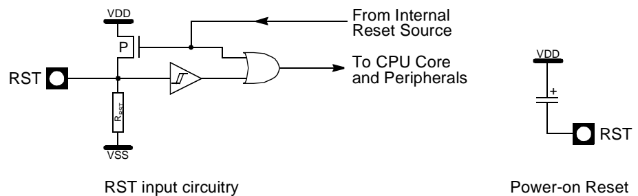
Figure 32. Reset Circuitry and Power-On Reset
