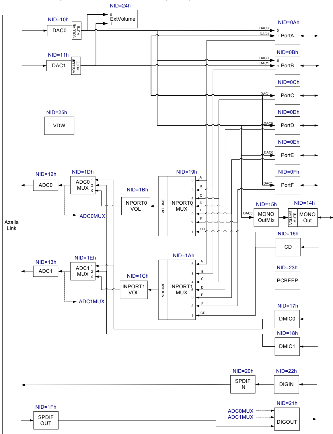
Figure 6. 92HD005/92HD005D Widget Diagram
