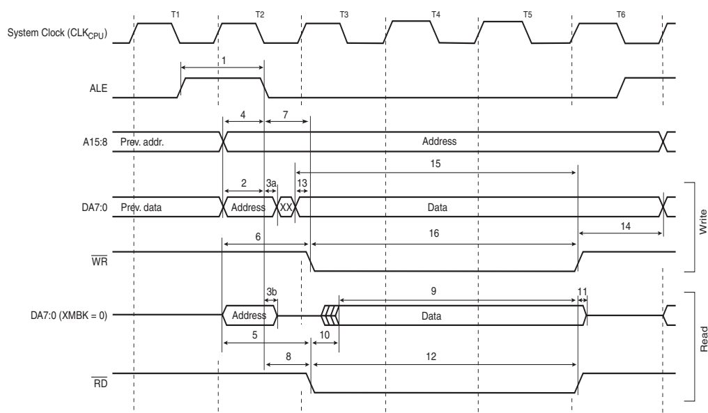
Figure 30-9. External Memory Timing (SRWn1 = 1, SRWn0 = 0)
