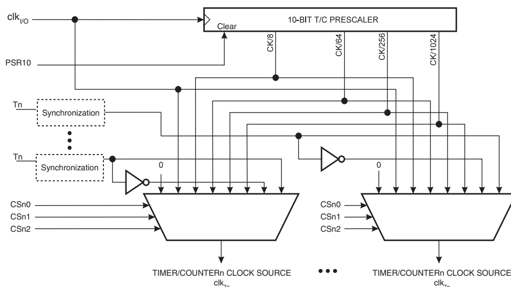
Figure 2. Prescaler for synchronous Timer/Counters
