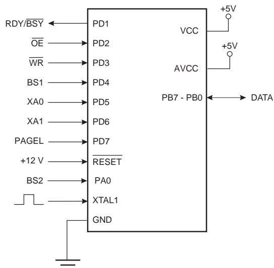
Figure 29-1. Parallel Programming (1)
