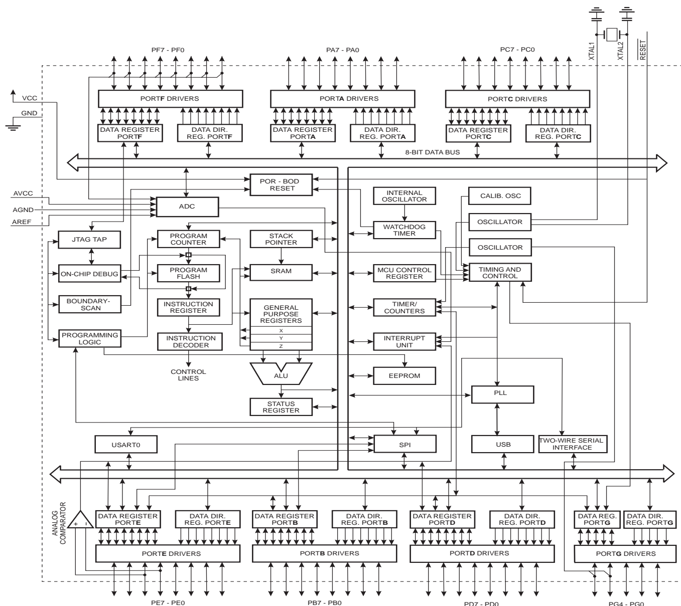
Figure 2-1. Block Diagram
