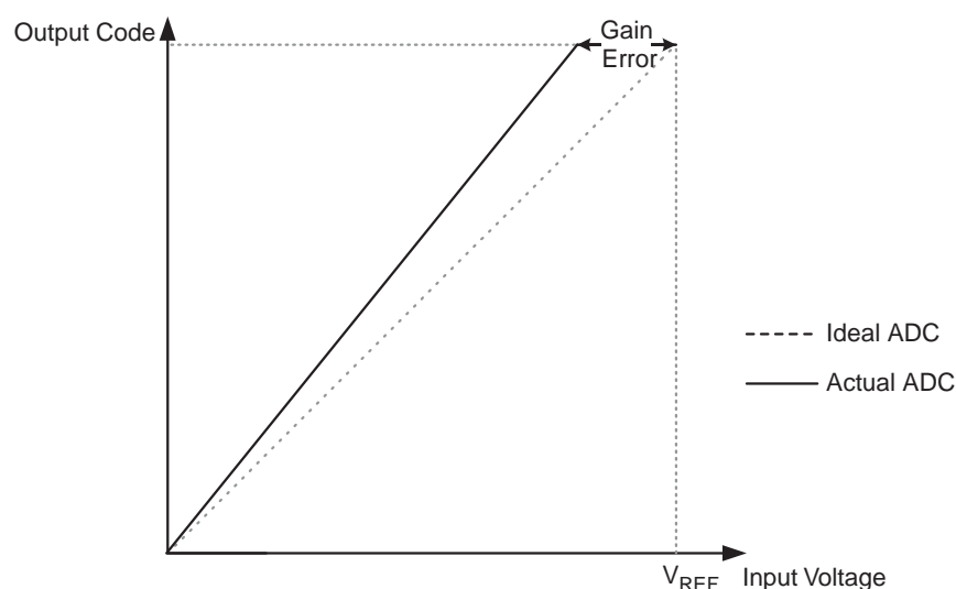
Figure 25-11. Gain Error
