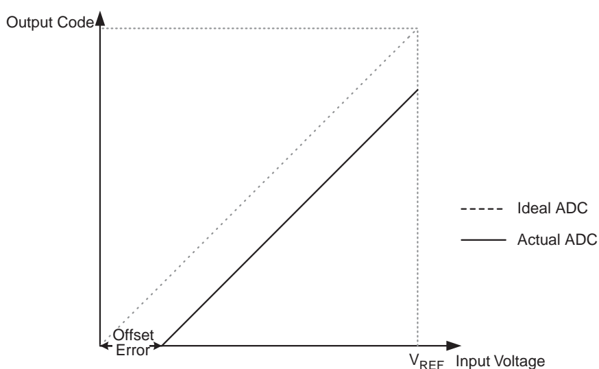
Figure 25-10. Offset Error
