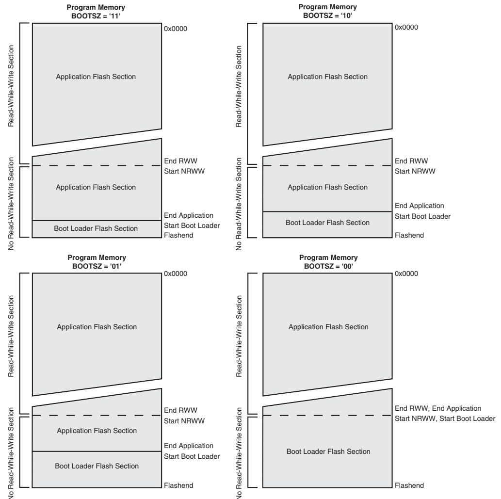
Figure 28-2. Memory Sections
