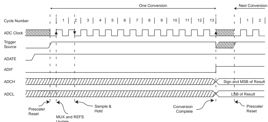
Figure 25-6. ADC Timing Diagram, Auto Triggered Conversion
