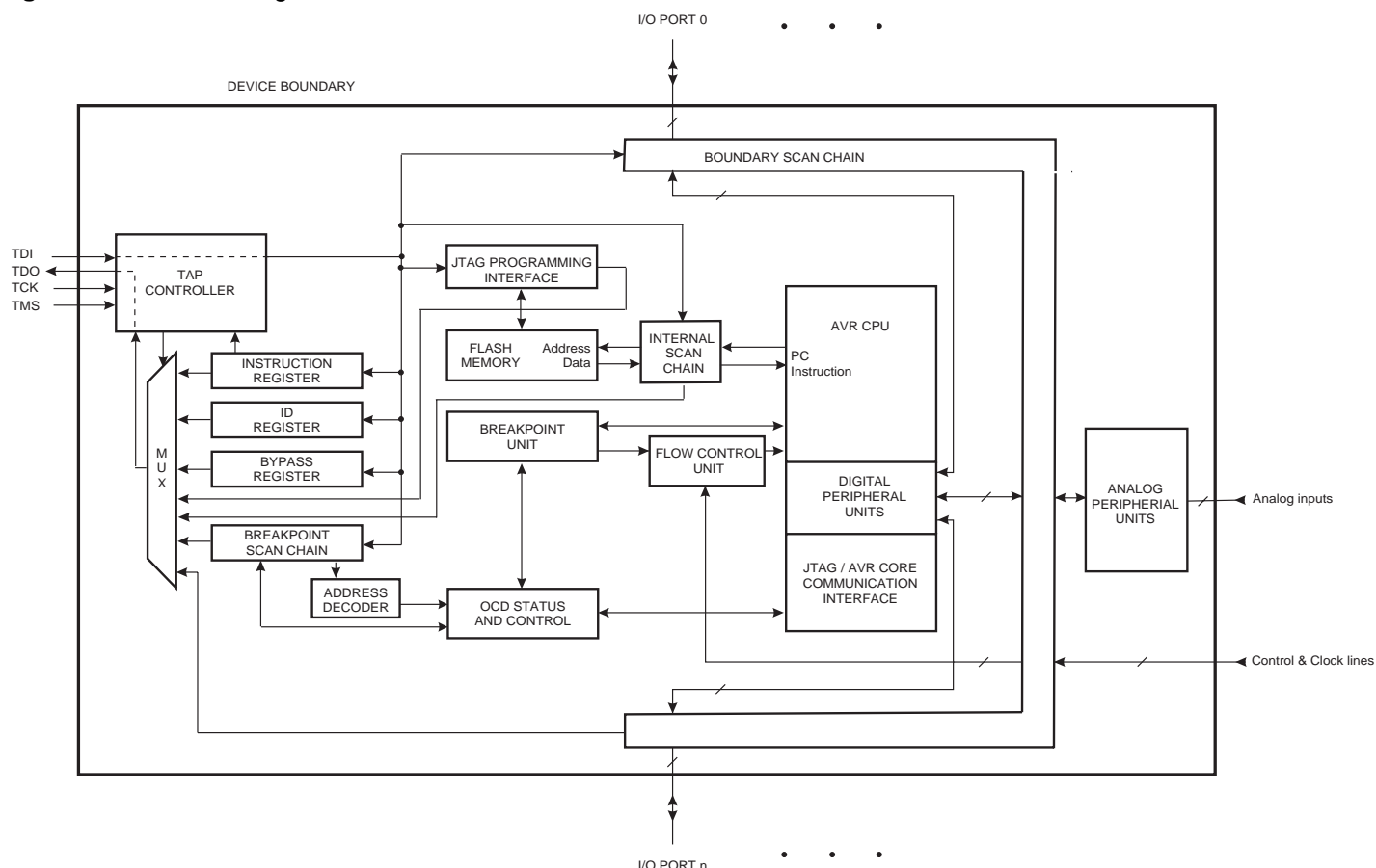
Figure 26-1. Block Diagram
