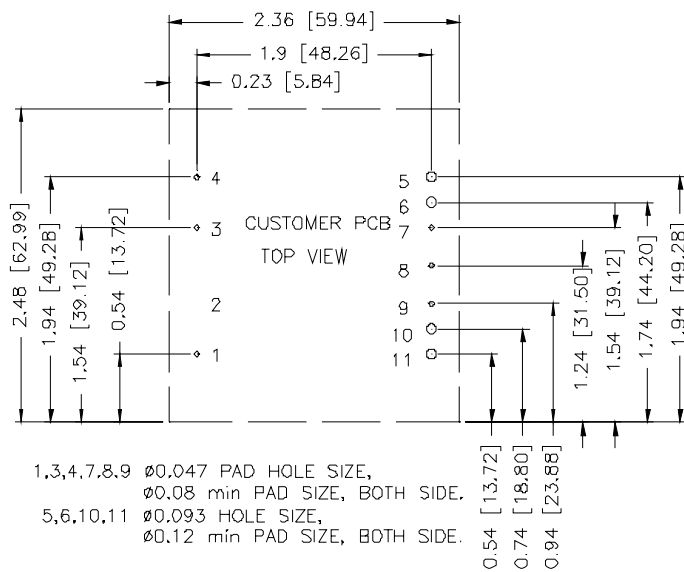
RECOMMENDED PAD LAYOUT
