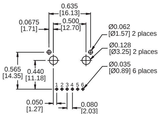
Suggested PCB Pad Layout
