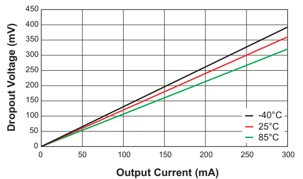
LDO2 Dropout Voltage vs. Output Current (V OUT2 = 3.4V)
