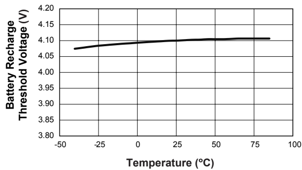
Battery Recharge Threshold Voltage vs. Temperature ( R_{\text{SENSE}} = 0.15\Omega )
