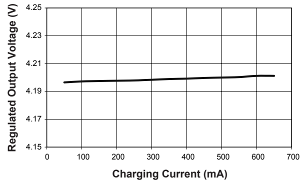
Regulated Output Voltage vs. Charge Current ( R_{\text{SENSE}} = 0.15\Omega )
