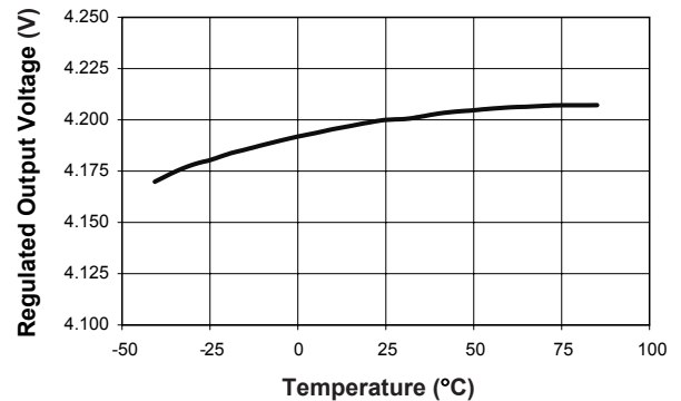
Regulated Output Voltage vs. Temperature ( R_{\text{SENSE}} = 0.15\Omega )
