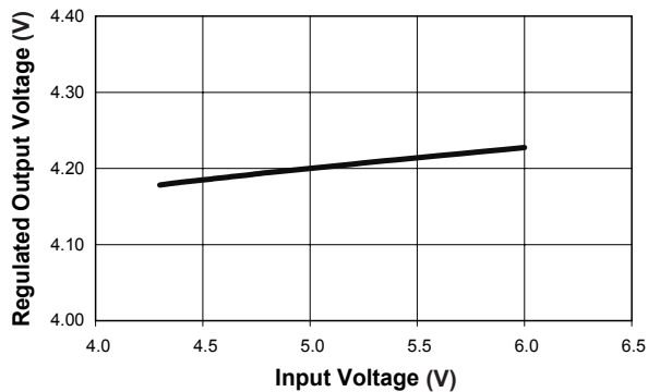
Regulated Output Voltage vs. Input Voltage ( R_{\text{SENSE}} = 0.15\Omega )
