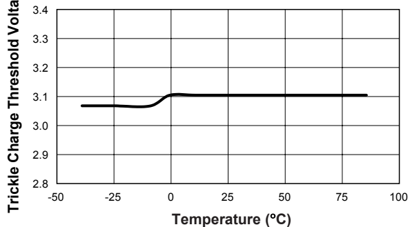
Trickle Charge Threshold Voltage vs. Temperature ( R_{\text{SENSE}} = 0.15\Omega )
