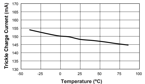
Trickle Charge Current vs. Temperature ( R_{\text{SENSE}} = 0.15\Omega )
