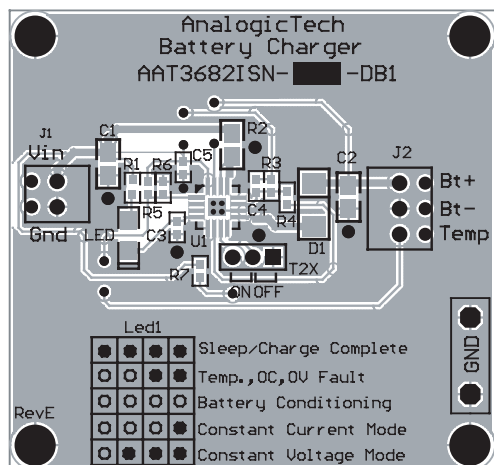
Figure 6: Evaluation Board Top Side Layout.
