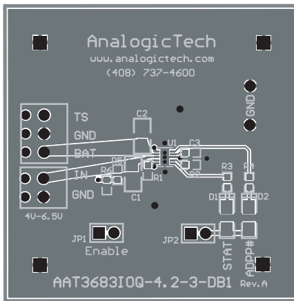
Figure 10: AAT3683-3 Evaluation Board Top Side Layout.
