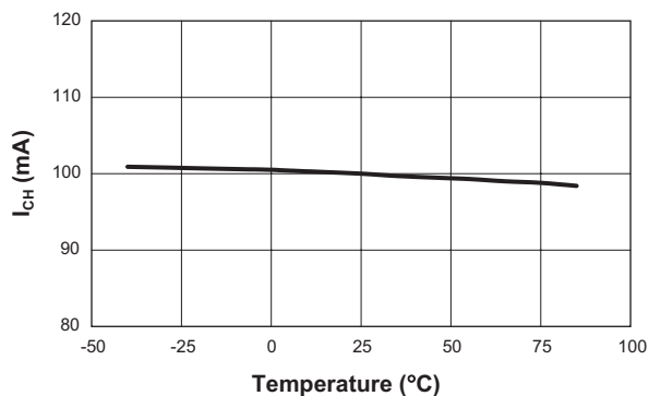
Preconditioning Charge Current vs. Temperature (SETH; R_{SET} = 3.83\text{k}\Omega )
