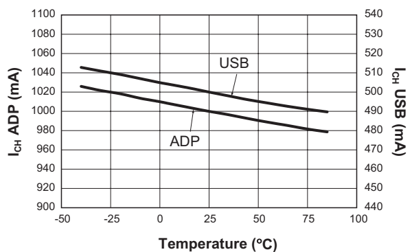
Fast Charge Current vs. Temperature ( R_{ADPSET} = 8.06\text{k}\Omega ; R_{USBSET} = 8.06\text{k}\Omega )
