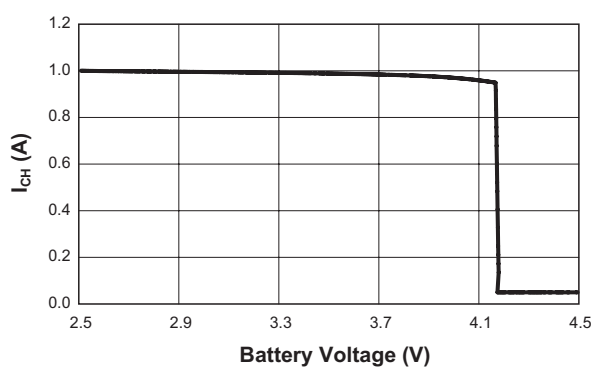
Adapter Charging Current vs. Battery Voltage ( R_{ADPSET} = 8.06\text{k}\Omega )
