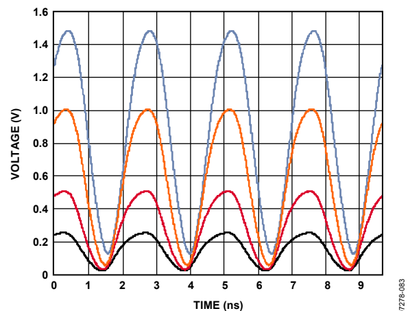
Figure 8. 400 MHz Driver Response; VH = 0.5 V, 1.0 V, 2.0 V, 3.0 V; VL = 0.0 V; 50 \Omega Termination
