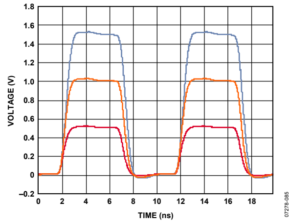
Figure 6. 100 MHz Driver Response; VH = 1.0 V, 2.0 V, 3.0 V; VL = 0.0 V; 50 \Omega Termination
