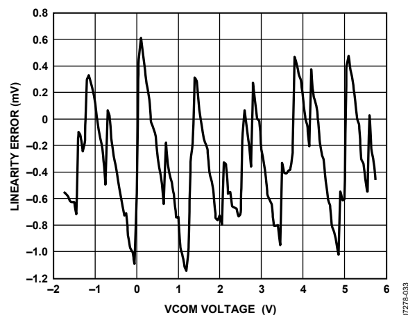
Figure 43. Active Load VCOM Linearity
