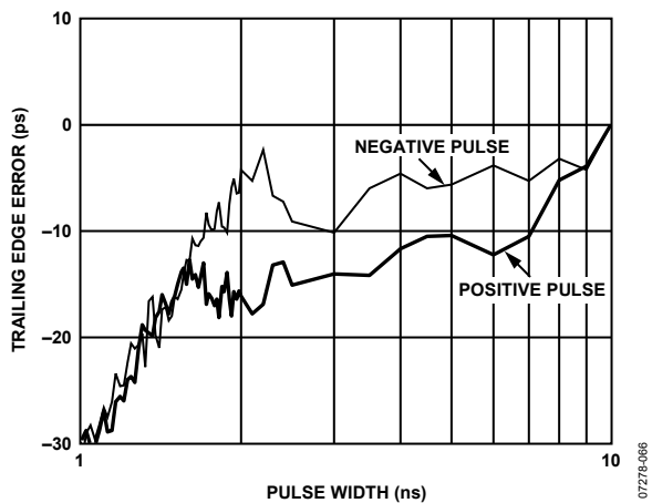
Figure 17. Driver Minimum Pulse Width; VH = 2.0 V; VL = 0.0 V
