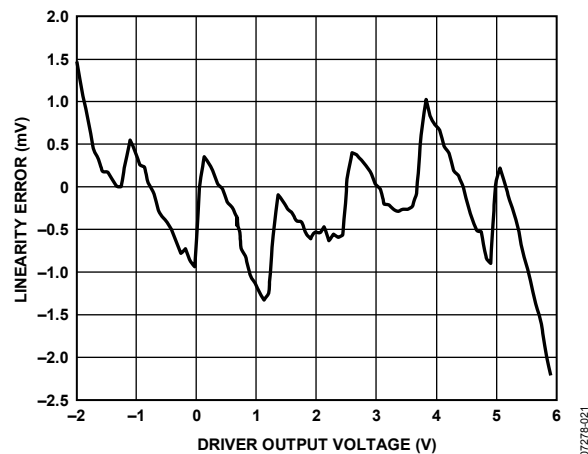
Figure 20. Driver VL Linearity Error
