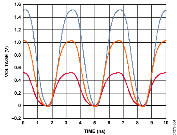
Figure 7. 300 MHz Driver Response; VH = 1.0 V, 2.0 V, 3.0 V; VL = 0.0 V; 50 \Omega Termination
