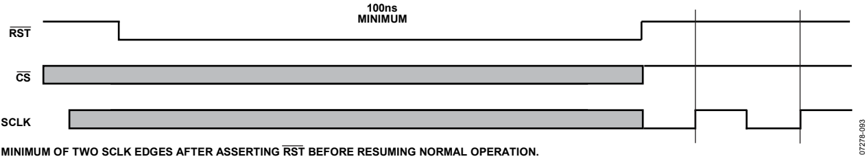
Figure 86. Reset Operation
