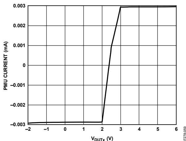
Figure 64. PMU Range E Internal Current Limit, Programmed to Force 2.5 V; V_{DUTx} Swept from -2.0 V to +6.0 V
