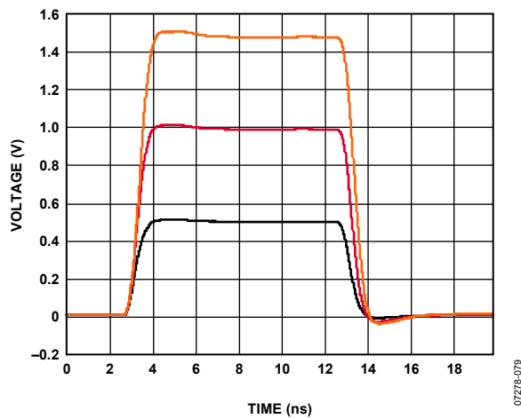
Figure 4. Driver Large Signal Response; VH = 1.0 V, 2.0 V, 3.0 V; VL = 0.0 V; 50 \Omega Termination
