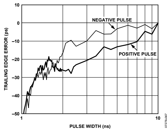
Figure 18. Driver Minimum Pulse Width; VH = 3.0 V; VL = 0.0 V
