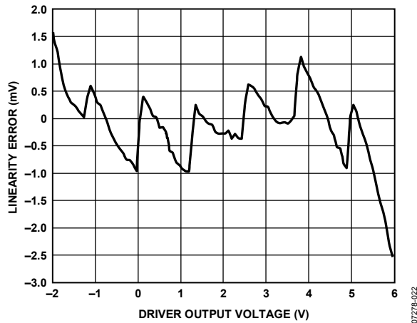
Figure 21. Driver VT Linearity Error
