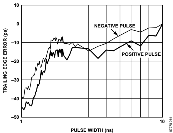
Figure 15. Driver Minimum Pulse Width; VH = 0.5 V; VL = 0.0 V
