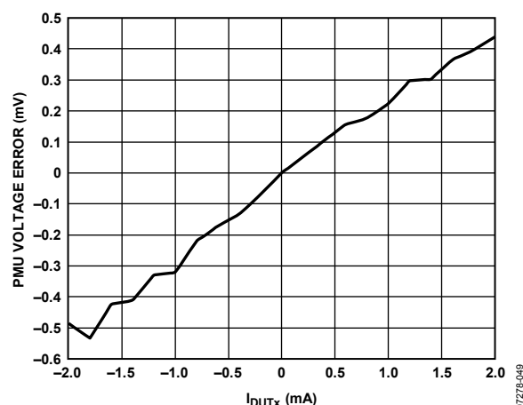
Figure 54. PMU Force Voltage Range B Output Voltage Error at -2.0 V vs. Output Current
