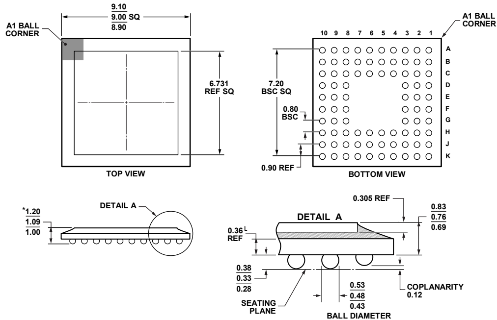
Figure 93. 84-Ball Chip Scale Package Ball Grid Array [CSP_BGA] (BC-84-2)
