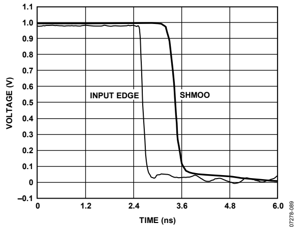
Figure 33. Comparator Shmoo; 1.0 V Swing; 200 ps (10%/90%)
