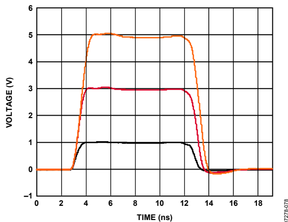
Figure 5. Driver Large Signal Response; VH = 1.0 V, 3.0 V, 5.0 V; VL = 0.0 V; 500 \Omega Termination
