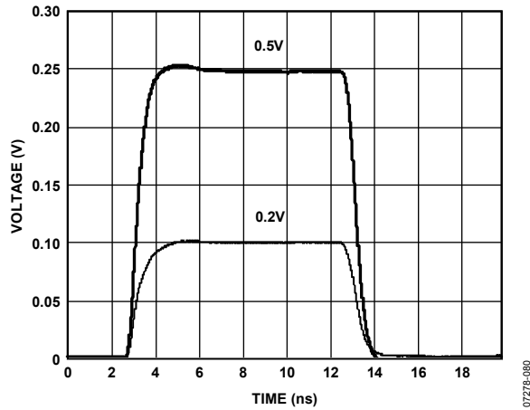
Figure 3. Driver Small Signal Response; VH = 0.2 V, 0.5 V; VL = 0.0 V; 50 \Omega Termination
