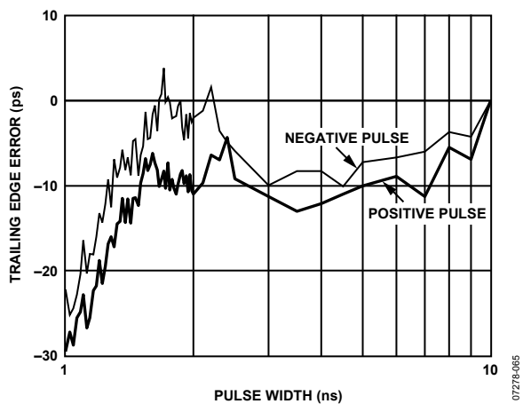
Figure 16. Driver Minimum Pulse Width; VH = 1.0 V; VL = 0.0 V
