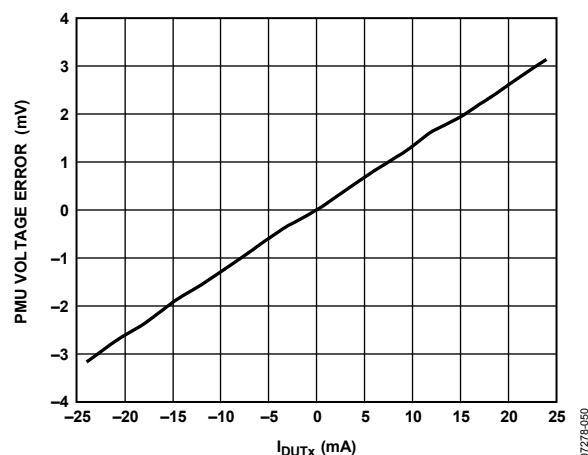
Figure 55. PMU Force Voltage Range A Output Voltage Error at 6.0 V vs. Output Current
