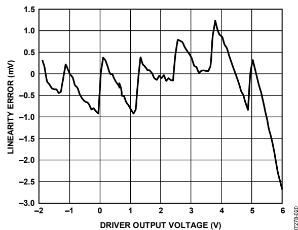
Figure 19. Driver VH Linearity Error
