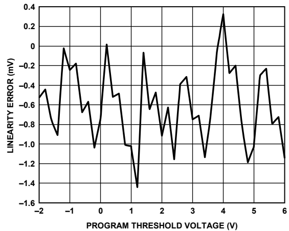
Figure 38. Comparator Threshold Linearity
