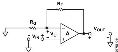
Figure 38. Noninverting Configuration
