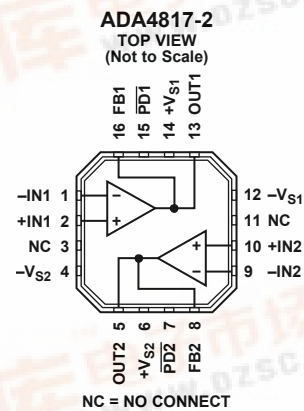
Figure 2. 16-Lead ADA4817-2 LFCSP (CP-16-4)
