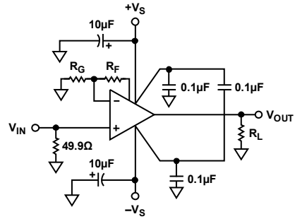
Figure 35. Noninverting Gain Configuration
