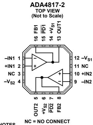
Figure 5. 16-Lead LFCSP Pin Configuration
