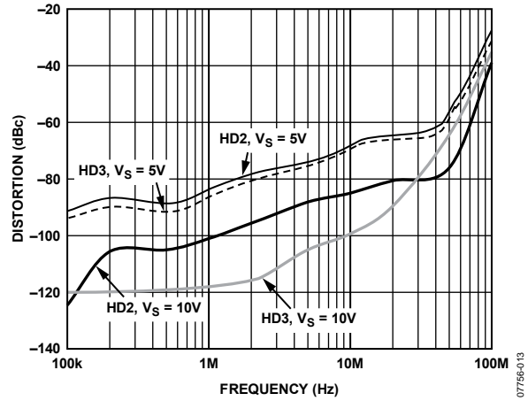
Figure 16. Distortion vs. Frequency for Various Supplies, V_{OUT} = 2V_{p-p}
