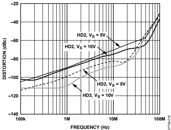
Figure 14. Distortion vs. Frequency for Various Supplies, G = 2 , V_{OUT} = 2V_{p-p}
