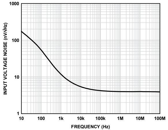
Figure 28. Input Voltage Noise
