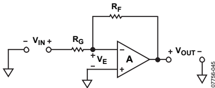
Figure 39. Inverting Configuration
