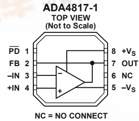
Figure 1. 8-Lead ADA4817-1 LFCSP (CP-8-2)
