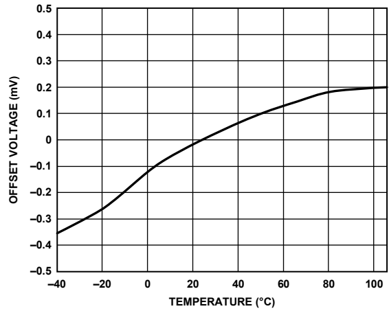
Figure 27. Offset Voltage vs. Temperature
