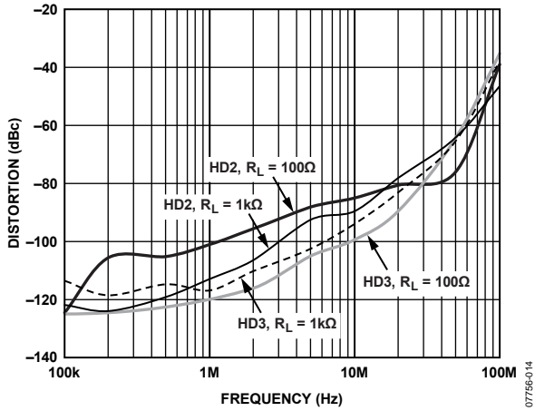
Figure 13. Distortion vs. Frequency for Various Loads, V_{OUT} = 2V_{p-p}
