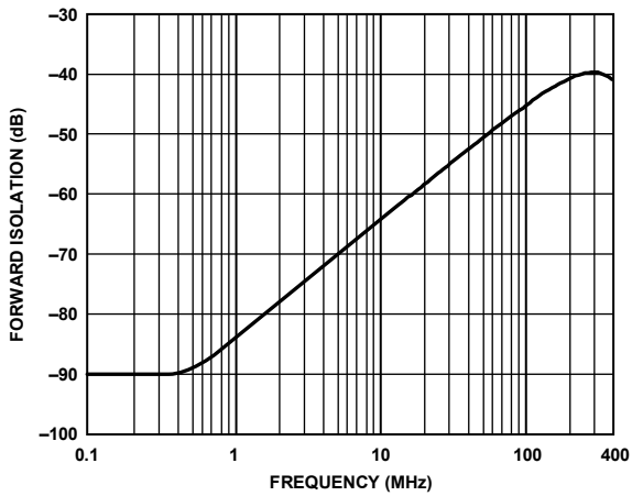
Figure 16. Forward Isolation vs. Frequency
