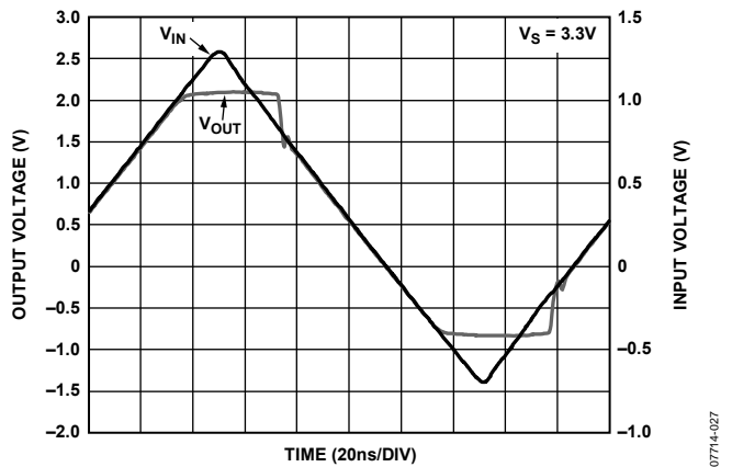
Figure 27. Output Overdrive Recovery, V_S = 3.3\text{ V}
