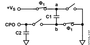
Figure 30. Charging Cycle
