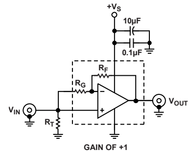
Figure 33. Unity Gain of Option 2
