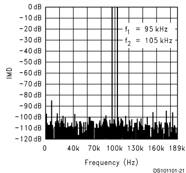
IMD Response
