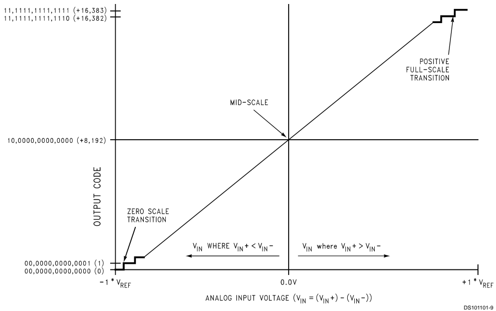
FIGURE 1. Transfer Characteristic
