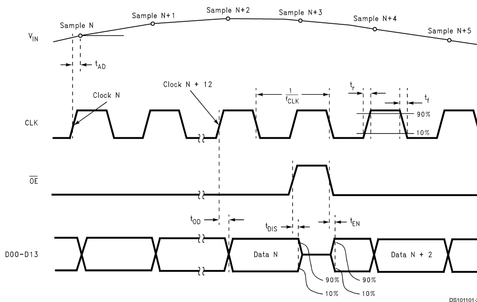
Output Timing
