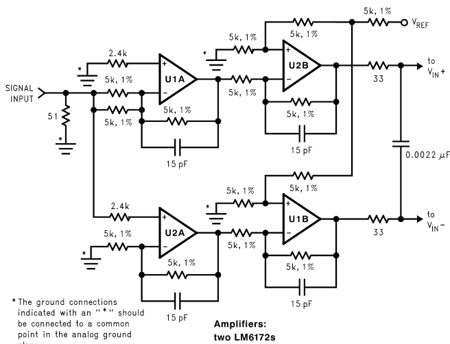
FIGURE 6. Differential Drive Circuit of Figure 5. All 100 \Omega Resistors are 0.1%. Tolerance of the other Resistors is not Critical.
