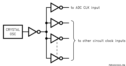
FIGURE 9. Isolating the ADC Clock from other Circuitry with A Clock Tree
