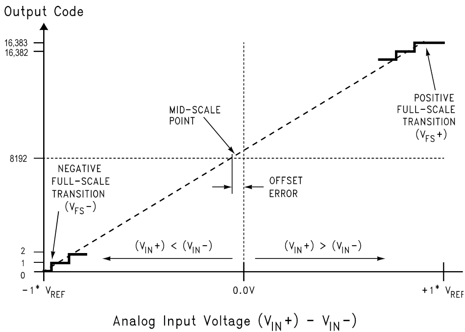
FIGURE 1. Transfer Characteristic
