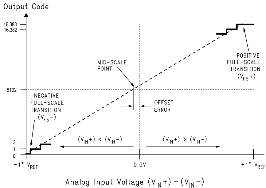
FIGURE 2. Transfer Characteristic
