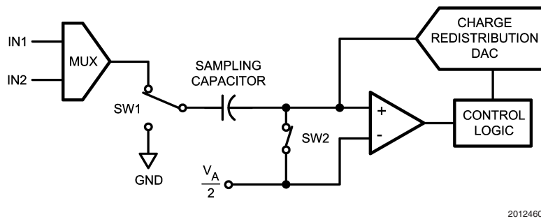
FIGURE 1. ADC122S021 in Track Mode
