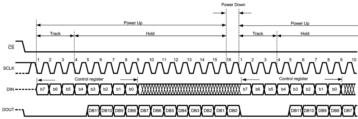
ADC122S021 Operational Timing Diagram
