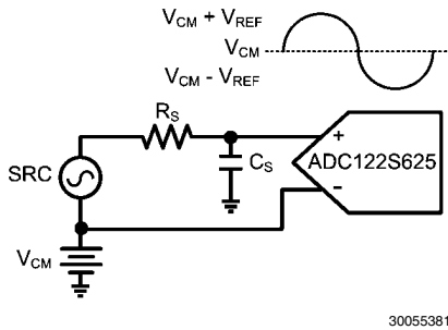
FIGURE 8. Single-Ended Input
