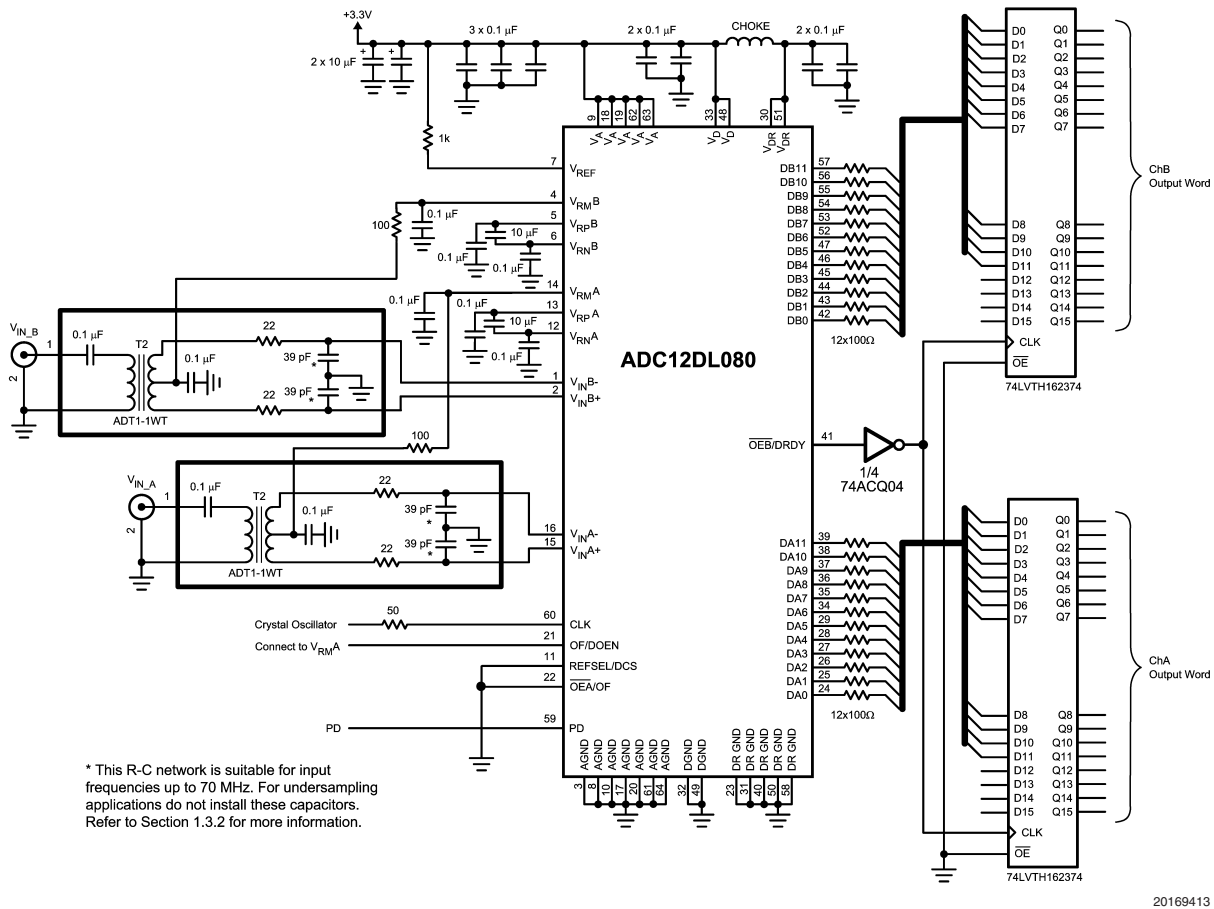
FIGURE 4. Application Circuit using Transformer Drive Circuit
