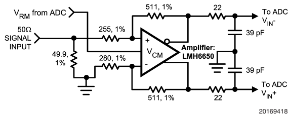
FIGURE 5. Optional Amplifier Drive for Circuit in Figure 4
