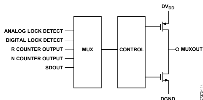
Figure 16. MUXOUT Circuit
