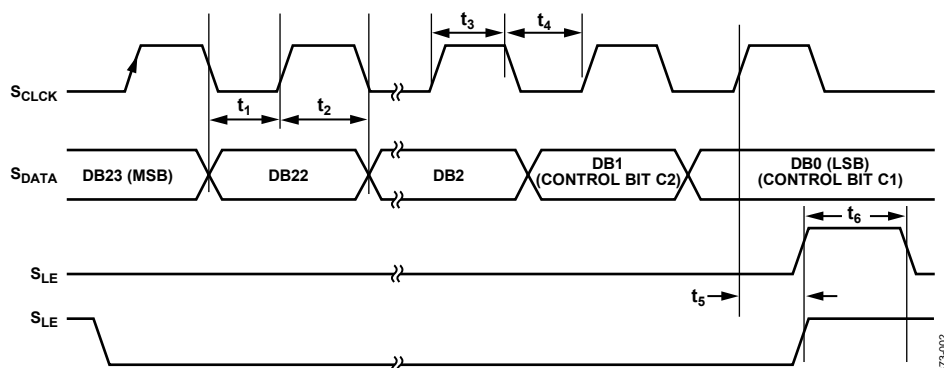
Figure 2. Write Timing Diagram
