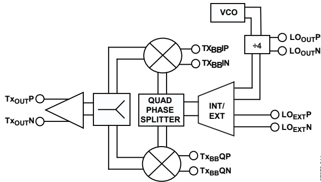
Figure 19. Tx Section
