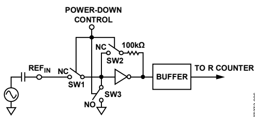
Figure 13. Reference Input Stage
