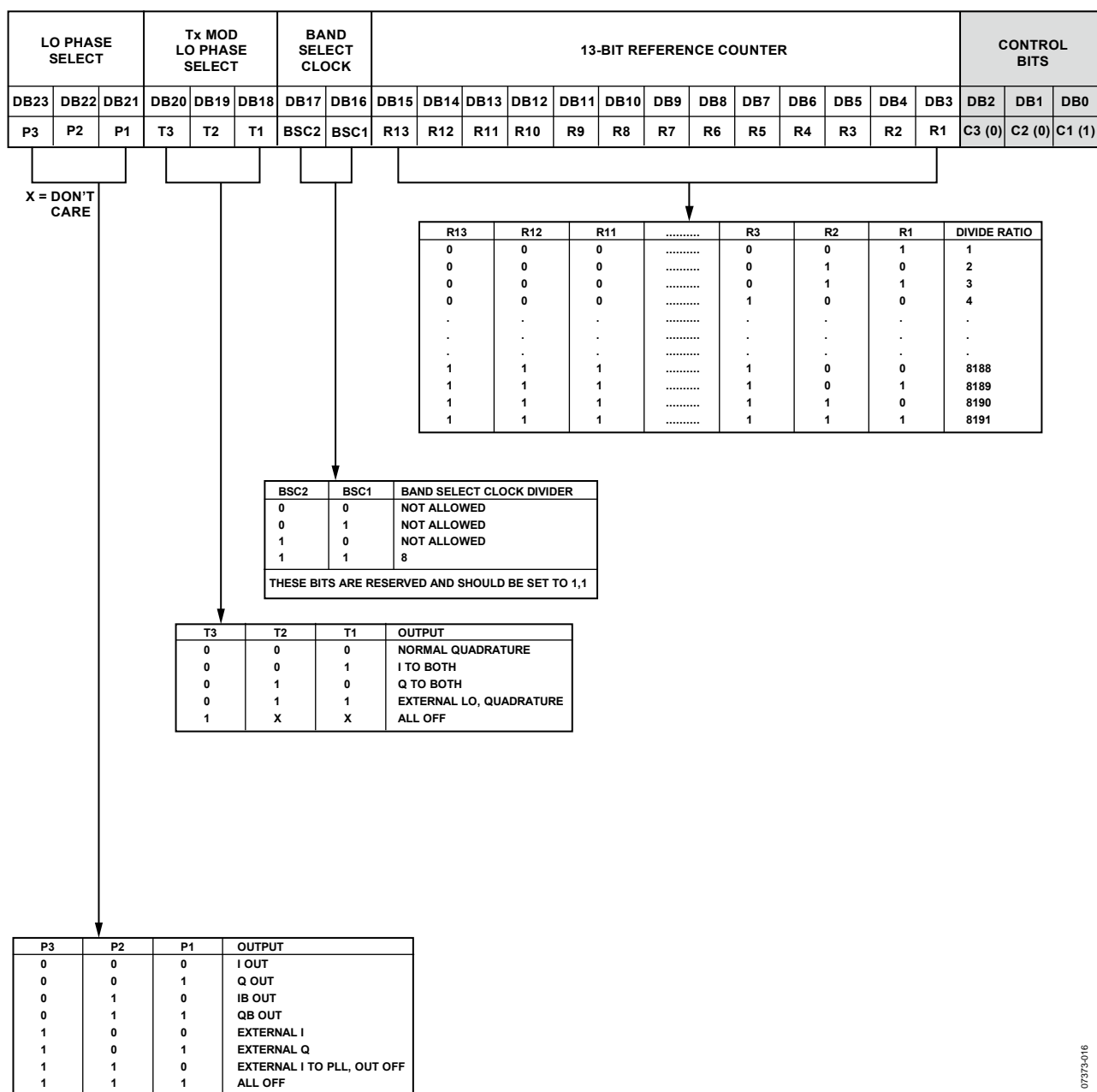
Figure 23. Tx Latch
