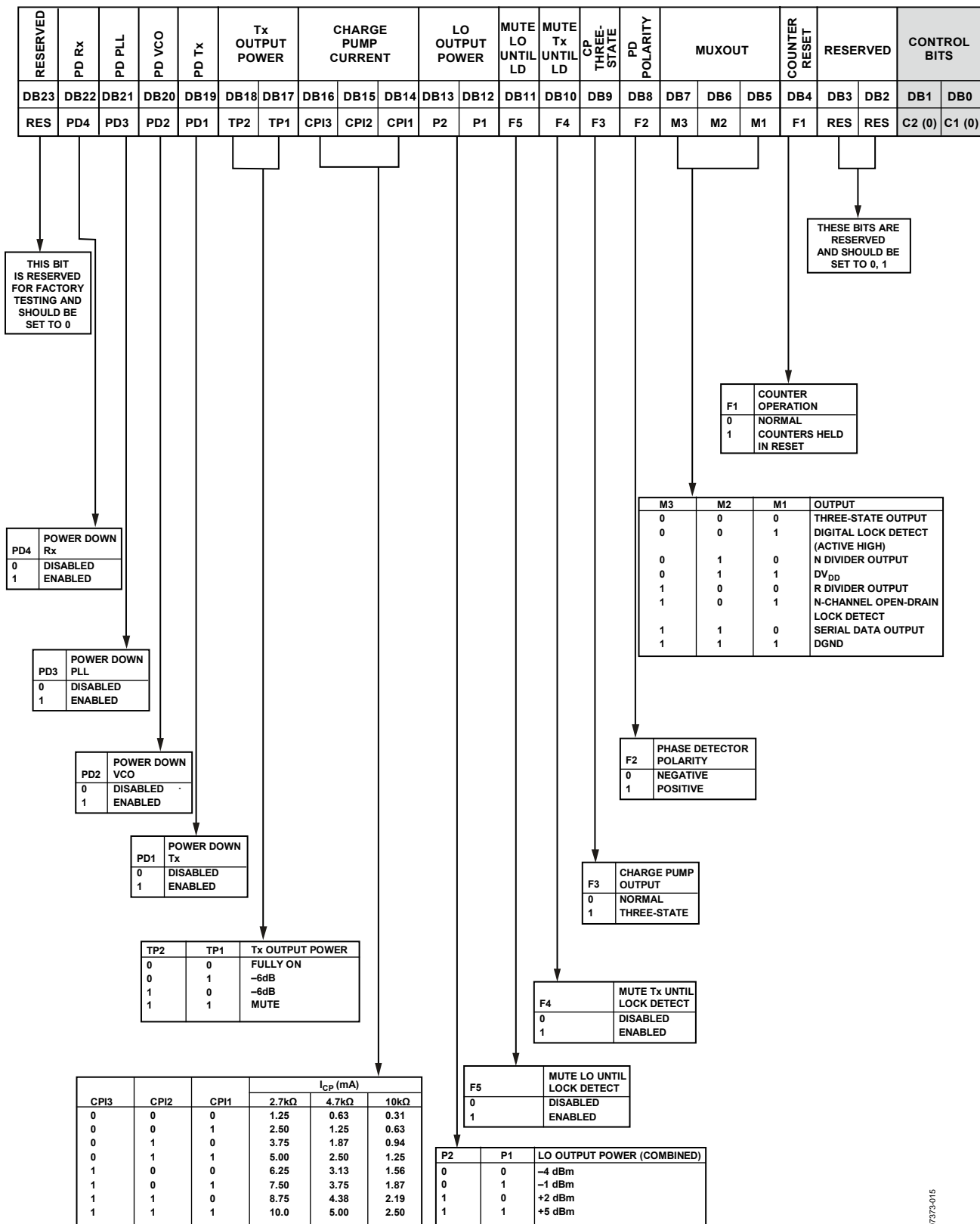
Figure 22. Control Latch
