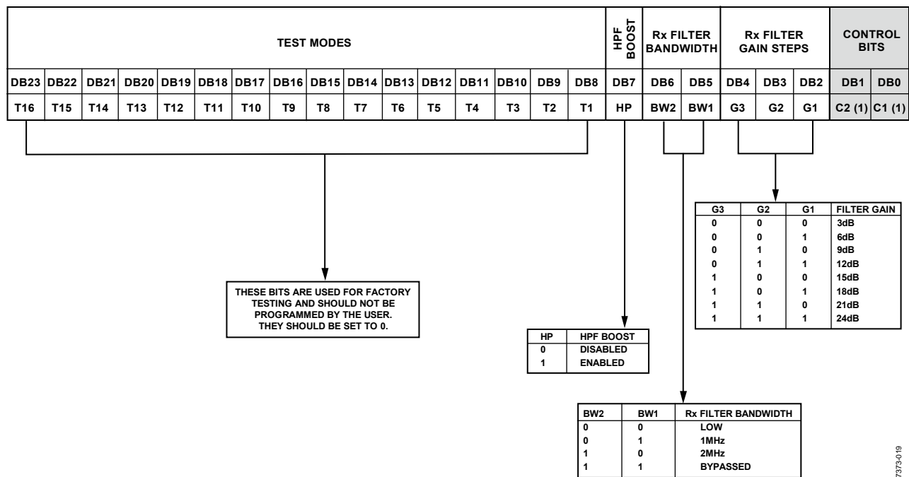
Figure 26. Rx Latch
