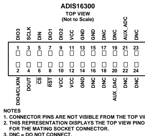
Figure 5. Pin Configuration
