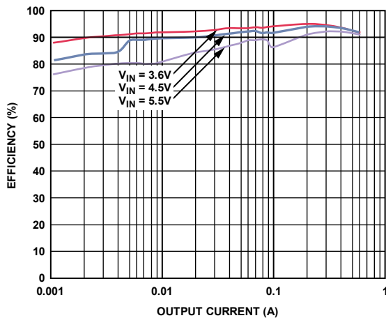
Figure 14. Efficiency, V_{OUT} = 3.3\text{ V}
