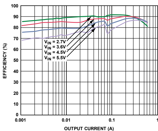
Figure 12. Efficiency, V_{OUT} = 1.8\text{ V}
