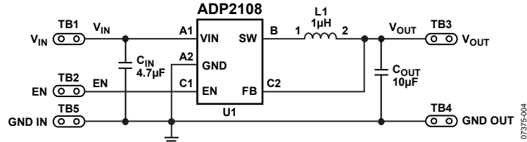
Figure 30. Evaluation Board Schematic
