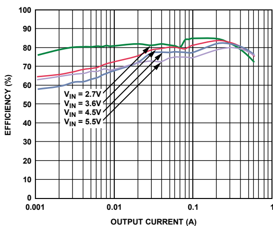
Figure 13. Efficiency, V_{OUT} = 1.0\text{ V}
