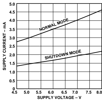
Figure 8. Supply Current vs. Supply Voltage
