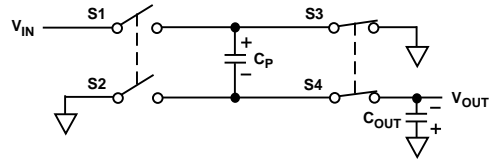
Figure 14. Switch Configuration Charging the Output Capacitor
