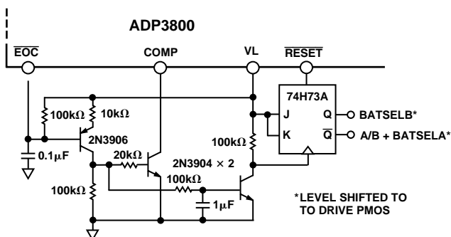
Figure 23. \overline{EOC} Output Circuits
