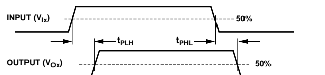
Figure 9. Propagation Delay Parameters
