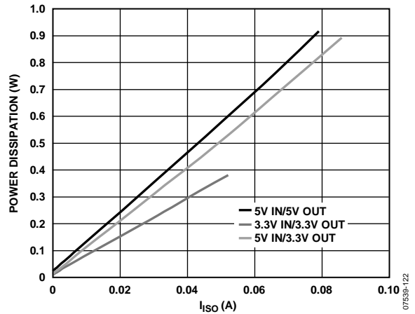
Figure 6. Typical Total Power Dissipation vs. I_{ISO} in All Supported Power Configurations
