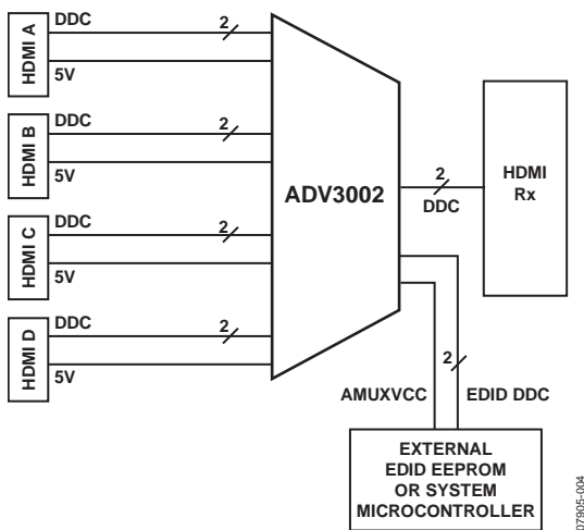
Figure 20. Simplified Implementation Using the ADV3002
