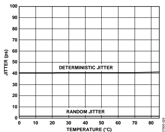
Figure 11. Jitter vs. Temperature
