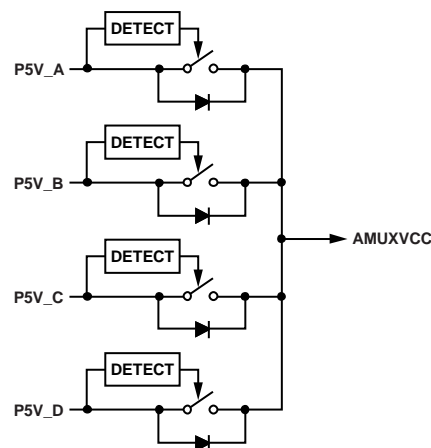
Figure 26. 5 V Combiner Simplified Circuit Diagram
