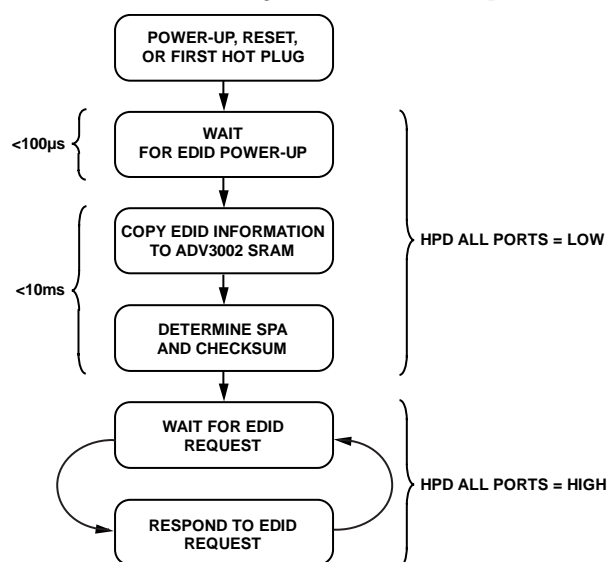
Figure 25. EDID Replication Start-Up Flowchart with External EEPROM
