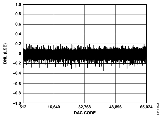
Figure 9. AD5065 DNL
