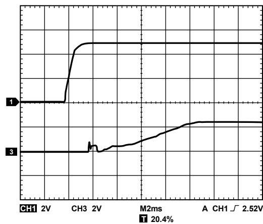
Figure 23. Power-On Reset to Midscale
