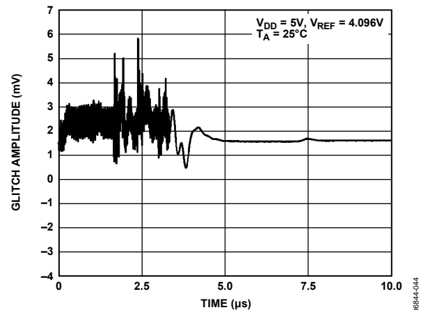
Figure 27. DAC-to-DAC Crosstalk
