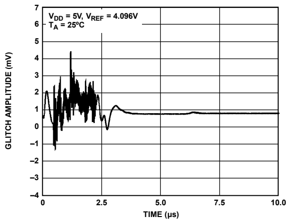
Figure 26. Analog Crosstalk
