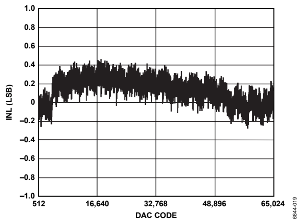
Figure 6. AD5065 INL
