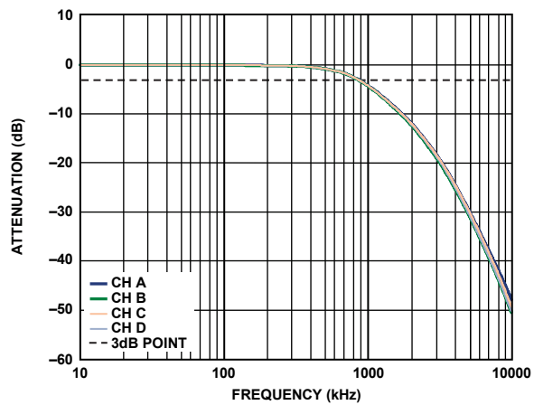
Figure 32. Multiplying Bandwidth
