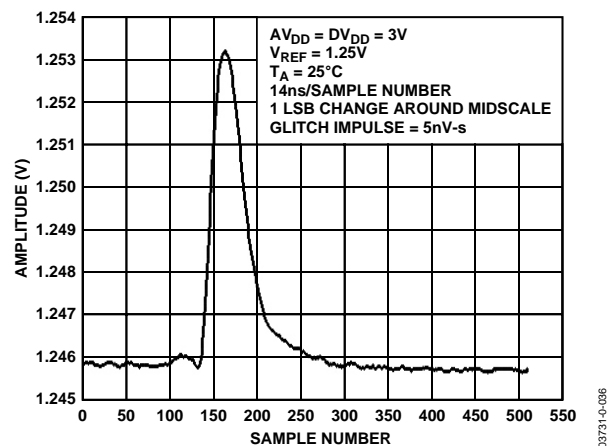
Figure 13. AD5382-3 Glitch Impulse
