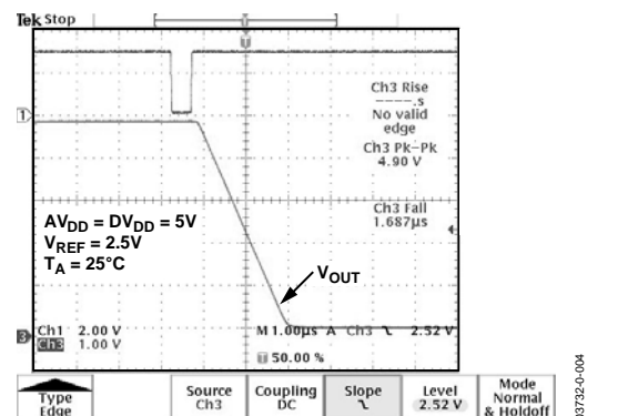
Figure 14. Slew Rate with Boost On
