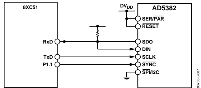
Figure 37. AD5382-to-8051 Interface
