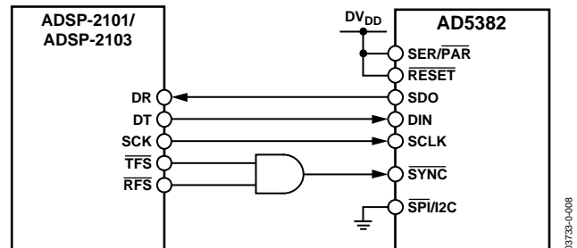
Figure 38. AD5382-to-ADSP-2101/ADSP-2103 Interface
